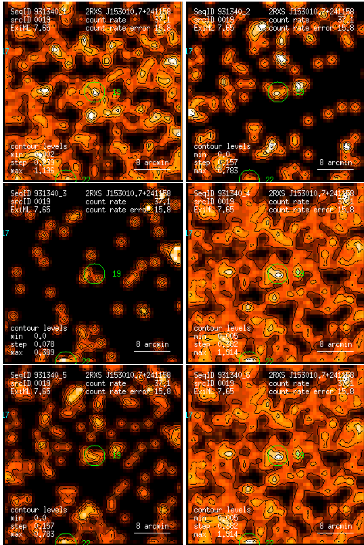
Figure 19: RASS 931340: detection 0019: band rate images, Gaussian filter: (1) PSPC channels 11 – 41, (2) 52 – 90, (3) 91 – 201, (4) 11 – 235, (5) 52 – 201, (6) 11 – 201. Broad band rates in counts/ks. Band rate contour levels in counts/ks/arcmin 2 .
