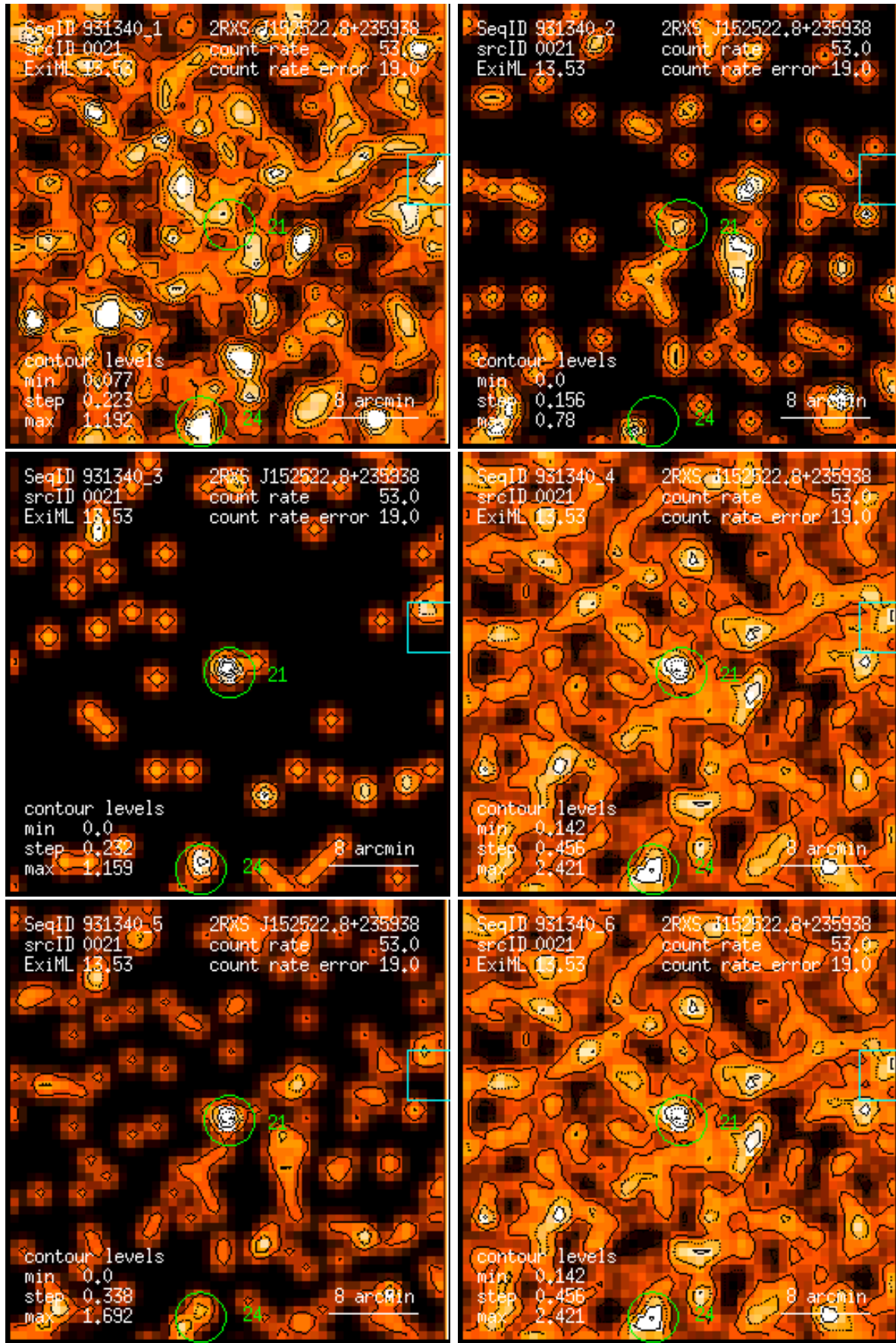
Figure 21: RASS 931340: detection 0021: band rate images, Gaussian filter: (1) PSPC channels 11 – 41, (2) 52 – 90, (3) 91 – 201, (4) 11 – 235, (5) 52 – 201, (6) 11 – 201. Broad band rates in counts/ks. Band rate contour levels in counts/ks/arcmin 2 .
