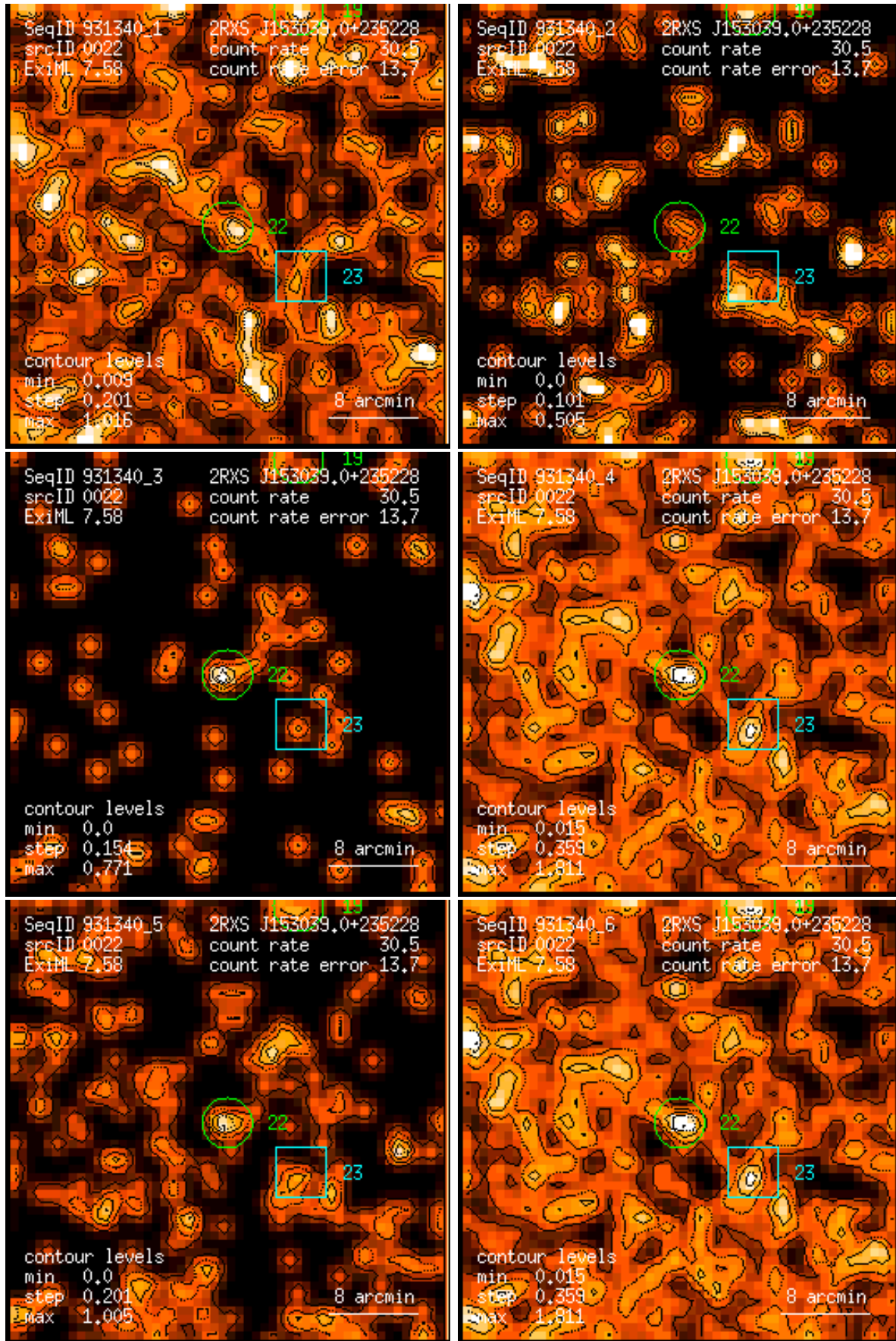
Figure 22: RASS 931340: detection 0022: band rate images, Gaussian filter: (1) PSPC channels 11 – 41, (2) 52 – 90, (3) 91 – 201, (4) 11 – 235, (5) 52 – 201, (6) 11 – 201. Broad band rates in counts/ks. Band rate contour levels in counts/ks/arcmin 2 .
