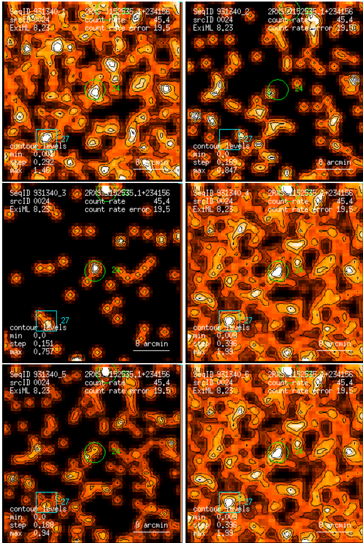
Figure 24: RASS 931340: detection 0024: band rate images, Gaussian filter: (1) PSPC channels 11 – 41, (2) 52 – 90, (3) 91 – 201, (4) 11 – 235, (5) 52 – 201, (6) 11 – 201. Broad band rates in counts/ks. Band rate contour levels in counts/ks/arcmin 2 .
