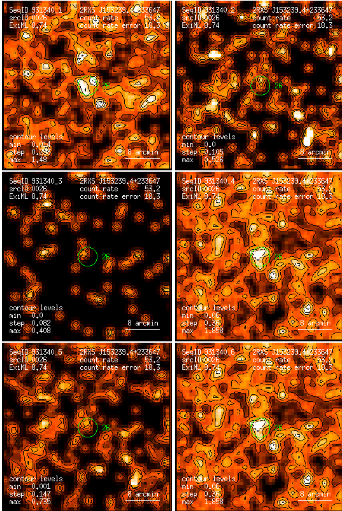
Figure 26: RASS 931340: detection 0026: band rate images, Gaussian filter: (1) PSPC channels 11 – 41, (2) 52 – 90, (3) 91 – 201, (4) 11 – 235, (5) 52 – 201, (6) 11 – 201. Broad band rates in counts/ks. Band rate contour levels in counts/ks/arcmin 2 .
