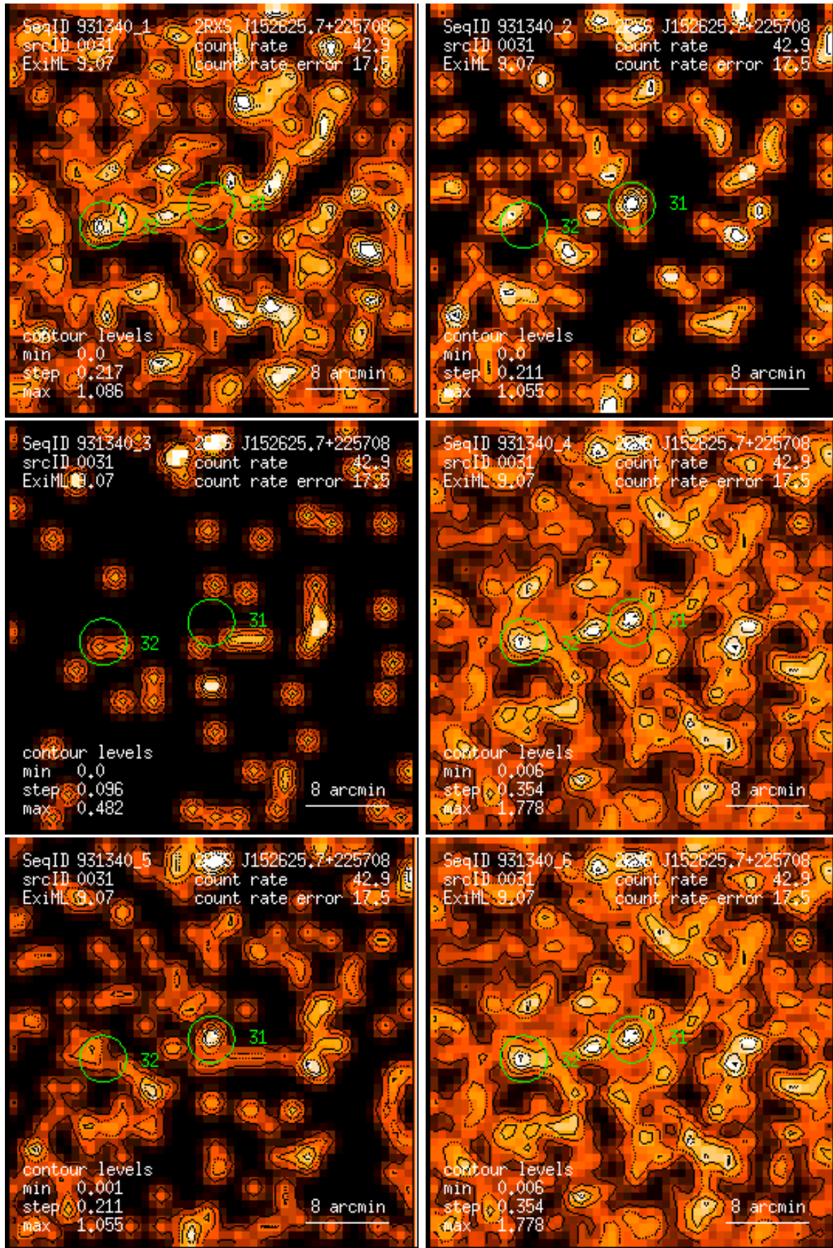
Figure 31: RASS 931340: detection 0031: band rate images, Gaussian filter: (1) PSPC channels 11 – 41, (2) 52 – 90, (3) 91 – 201, (4) 11 – 235, (5) 52 – 201, (6) 11 – 201. Broad band rates in counts/ks. Band rate contour levels in counts/ks/arcmin 2 .
