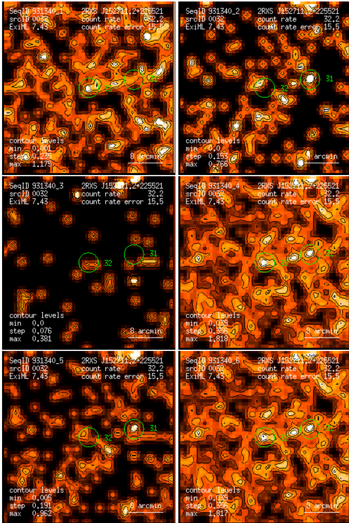
Figure 32: RASS 931340: detection 0032: band rate images, Gaussian filter: (1) PSPC channels 11 – 41, (2) 52 – 90, (3) 91 – 201, (4) 11 – 235, (5) 52 – 201, (6) 11 – 201. Broad band rates in counts/ks. Band rate contour levels in counts/ks/arcmin 2 .
