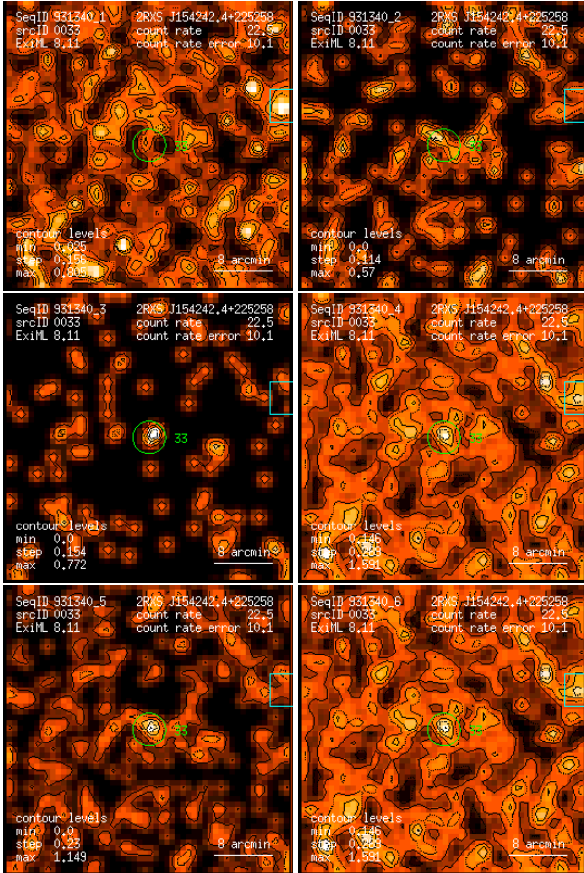
Figure 33: RASS 931340: detection 0033: band rate images, Gaussian filter: (1) PSPC channels 11 – 41, (2) 52 – 90, (3) 91 – 201, (4) 11 – 235, (5) 52 – 201, (6) 11 – 201. Broad band rates in counts/ks. Band rate contour levels in counts/ks/arcmin 2 .
