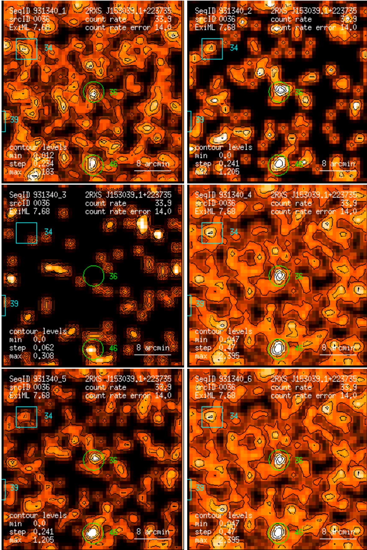
Figure 36: RASS 931340: detection 0036: band rate images, Gaussian filter: (1) PSPC channels 11 – 41, (2) 52 – 90, (3) 91 – 201, (4) 11 – 235, (5) 52 – 201, (6) 11 – 201. Broad band rates in counts/ks. Band rate contour levels in counts/ks/arcmin 2 .
