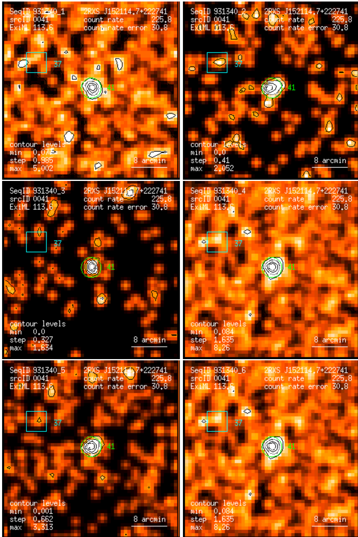
Figure 41: RASS 931340: detection 0041: band rate images, Gaussian filter: (1) PSPC channels 11 – 41, (2) 52 – 90, (3) 91 – 201, (4) 11 – 235, (5) 52 – 201, (6) 11 – 201. Broad band rates in counts/ks. Band rate contour levels in counts/ks/arcmin 2 .
