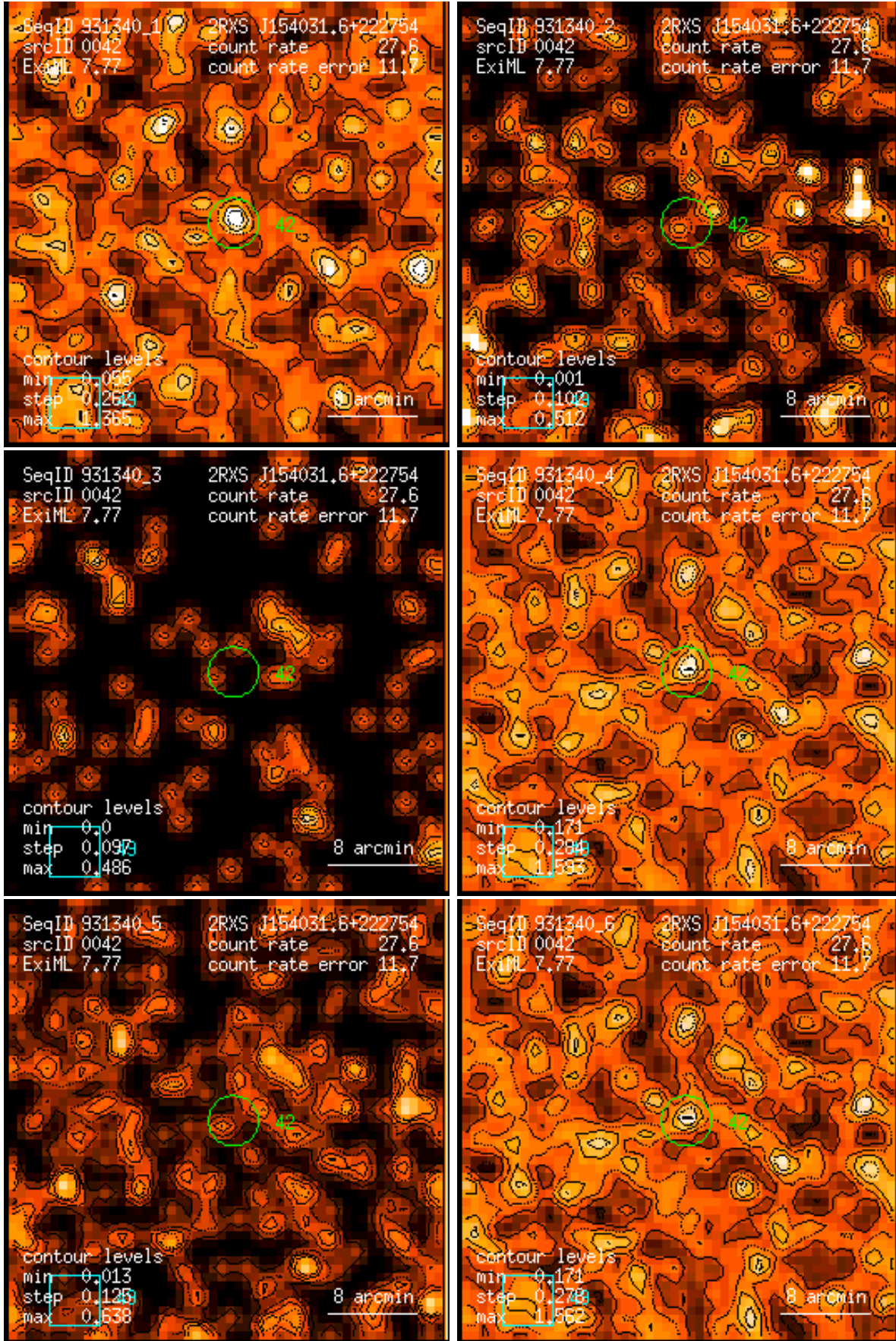
Figure 42: RASS 931340: detection 0042: band rate images, Gaussian filter: (1) PSPC channels 11 – 41, (2) 52 – 90, (3) 91 – 201, (4) 11 – 235, (5) 52 – 201, (6) 11 – 201. Broad band rates in counts/ks. Band rate contour levels in counts/ks/arcmin 2 .
