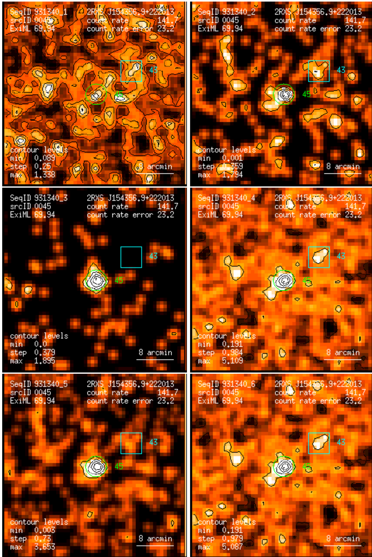
Figure 45: RASS 931340: detection 0045: band rate images, Gaussian filter: (1) PSPC channels 11 – 41, (2) 52 – 90, (3) 91 – 201, (4) 11 – 235, (5) 52 – 201, (6) 11 – 201. Broad band rates in counts/ks. Band rate contour levels in counts/ks/arcmin 2 .
