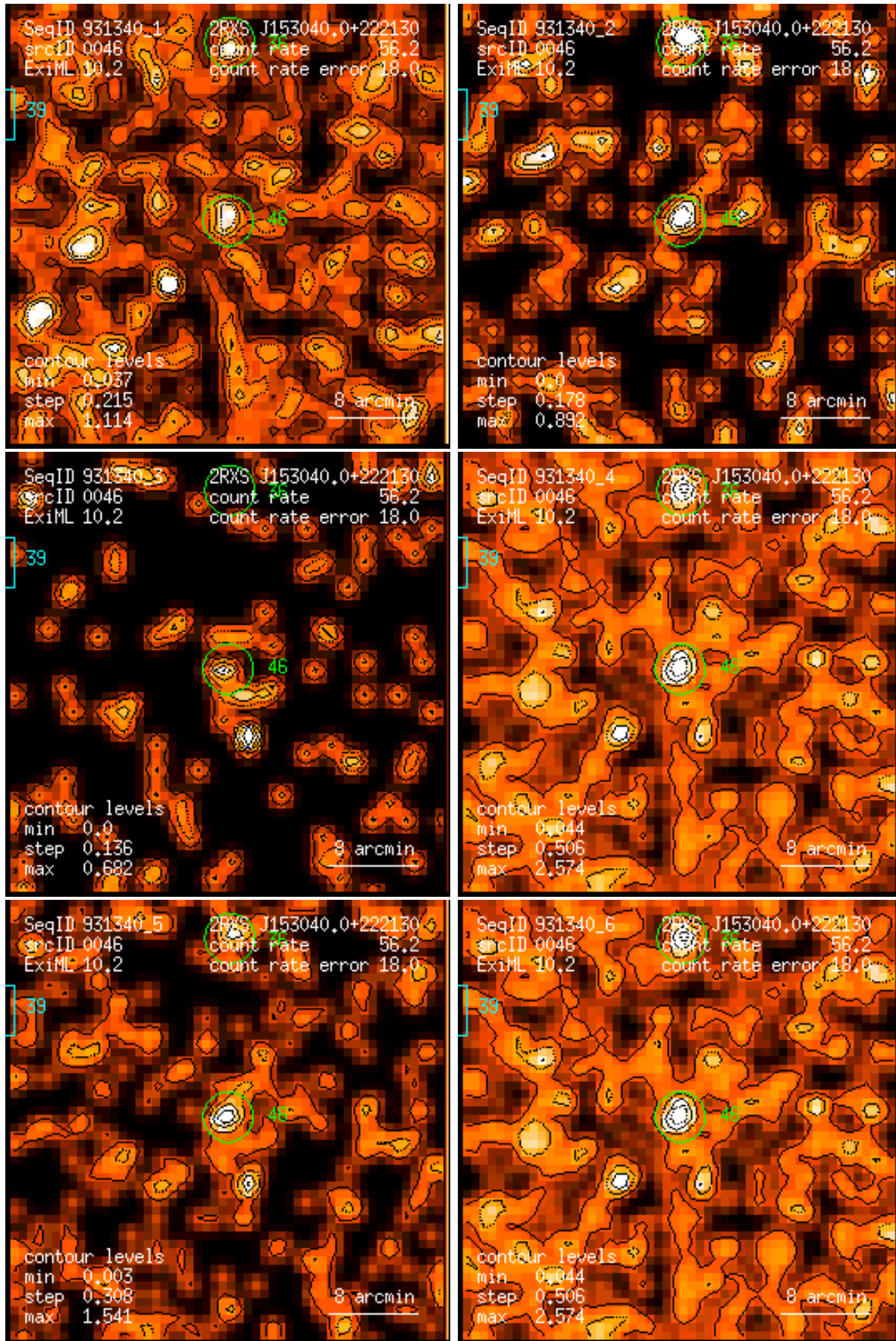
Figure 46: RASS 931340: detection 0046: band rate images, Gaussian filter: (1) PSPC channels 11 – 41, (2) 52 – 90, (3) 91 – 201, (4) 11 – 235, (5) 52 – 201, (6) 11 – 201. Broad band rates in counts/ks. Band rate contour levels in counts/ks/arcmin 2 .
