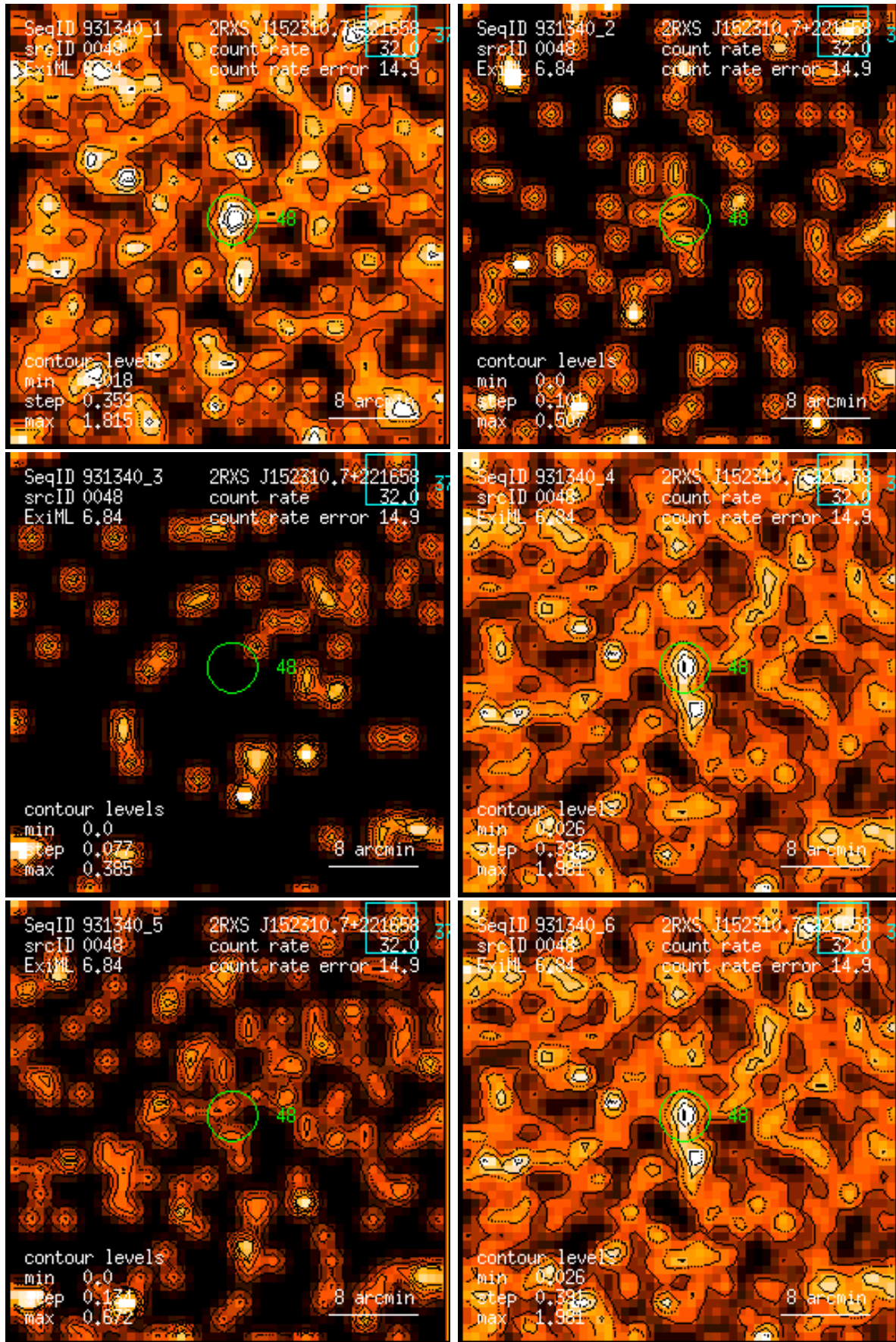
Figure 48: RASS 931340: detection 0048: band rate images, Gaussian filter: (1) PSPC channels 11 – 41, (2) 52 – 90, (3) 91 – 201, (4) 11 – 235, (5) 52 – 201, (6) 11 – 201. Broad band rates in counts/ks. Band rate contour levels in counts/ks/arcmin 2 .
