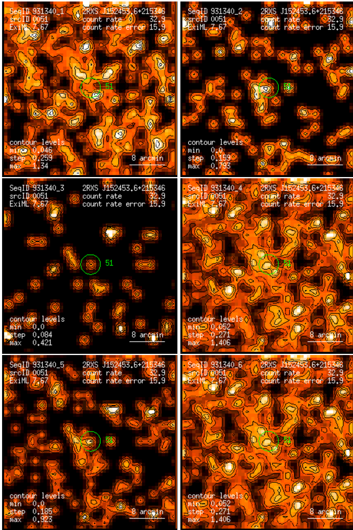
Figure 51: RASS 931340: detection 0051: band rate images, Gaussian filter: (1) PSPC channels 11 – 41, (2) 52 – 90, (3) 91 – 201, (4) 11 – 235, (5) 52 – 201, (6) 11 – 201. Broad band rates in counts/ks. Band rate contour levels in counts/ks/arcmin 2 .
