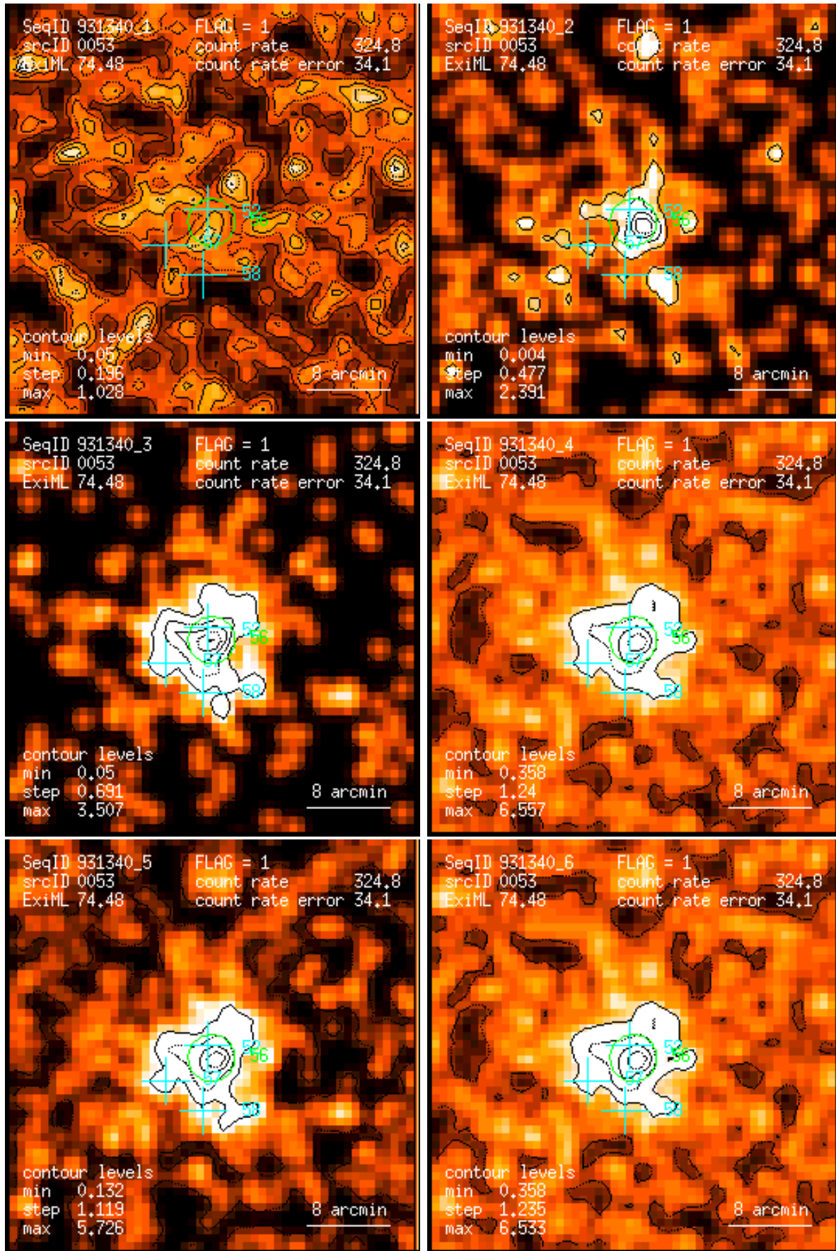
Figure 53: RASS 931340: detection 0053: band rate images, Gaussian filter: (1) PSPC channels 11 – 41, (2) 52 – 90, (3) 91 – 201, (4) 11 – 235, (5) 52 – 201, (6) 11 – 201. Broad band rates in counts/ks. Band rate contour levels in counts/ks/arcmin 2 .
