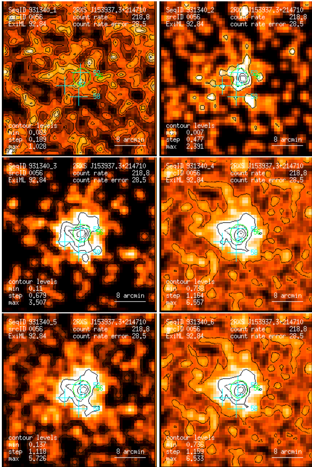
Figure 56: RASS 931340: detection 0056: band rate images, Gaussian filter: (1) PSPC channels 11 – 41, (2) 52 – 90, (3) 91 – 201, (4) 11 – 235, (5) 52 – 201, (6) 11 – 201. Broad band rates in counts/ks. Band rate contour levels in counts/ks/arcmin 2 .
