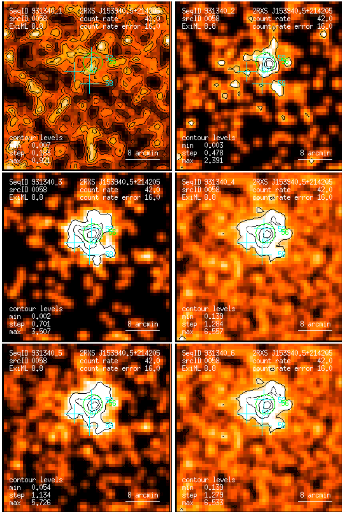
Figure 58: RASS 931340: detection 0058: band rate images, Gaussian filter: (1) PSPC channels 11 – 41, (2) 52 – 90, (3) 91 – 201, (4) 11 – 235, (5) 52 – 201, (6) 11 – 201. Broad band rates in counts/ks. Band rate contour levels in counts/ks/arcmin 2 .
