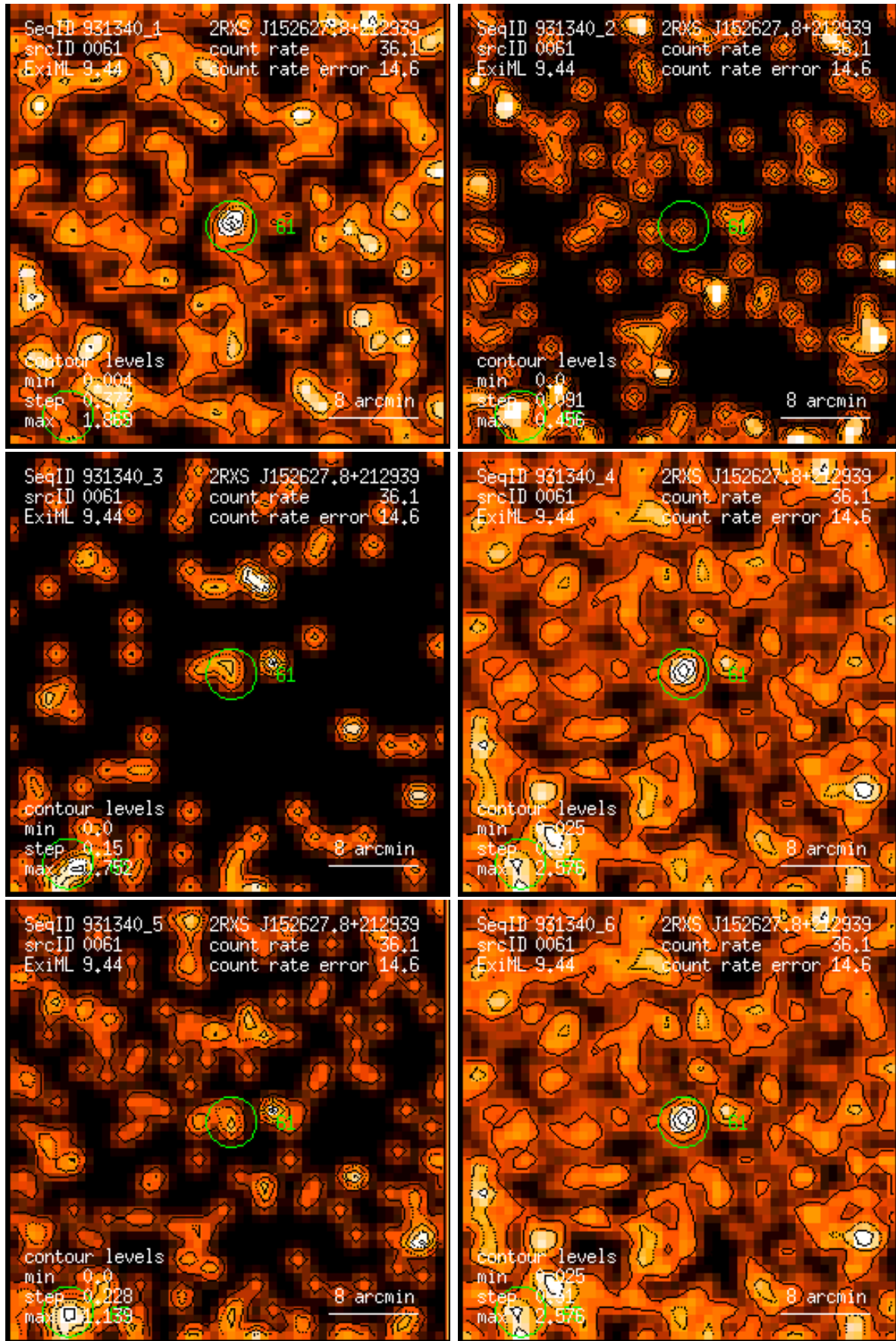
Figure 61: RASS 931340: detection 0061: band rate images, Gaussian filter: (1) PSPC channels 11 – 41, (2) 52 – 90, (3) 91 – 201, (4) 11 – 235, (5) 52 – 201, (6) 11 – 201. Broad band rates in counts/ks. Band rate contour levels in counts/ks/arcmin 2 .
