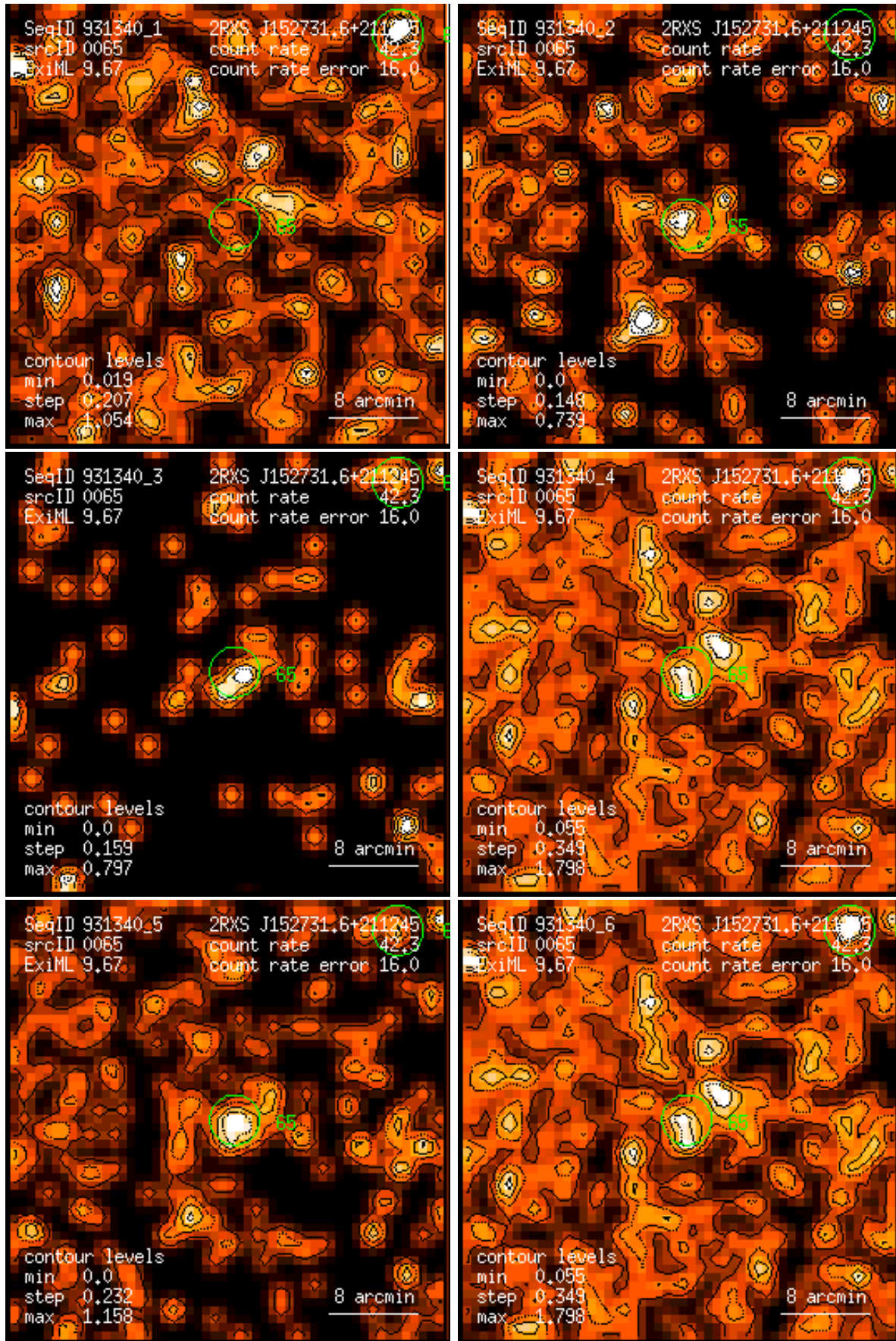
Figure 65: RASS 931340: detection 0065: band rate images, Gaussian filter: (1) PSPC channels 11 – 41, (2) 52 – 90, (3) 91 – 201, (4) 11 – 235, (5) 52 – 201, (6) 11 – 201. Broad band rates in counts/ks. Band rate contour levels in counts/ks/arcmin 2 .
