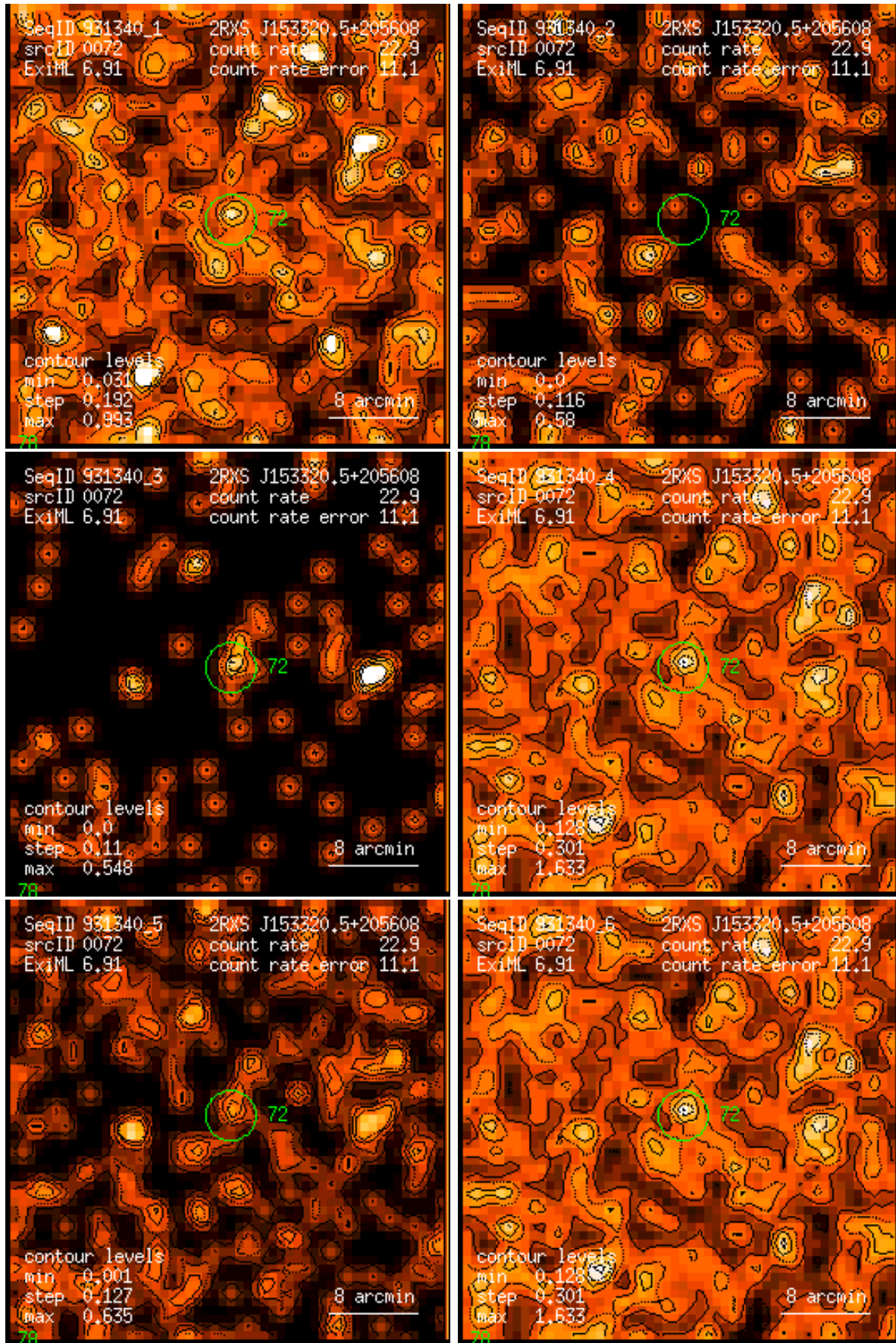
Figure 72: RASS 931340: detection 0072: band rate images, Gaussian filter: (1) PSPC channels 11 – 41, (2) 52 – 90, (3) 91 – 201, (4) 11 – 235, (5) 52 – 201, (6) 11 – 201. Broad band rates in counts/ks. Band rate contour levels in counts/ks/arcmin 2 .
