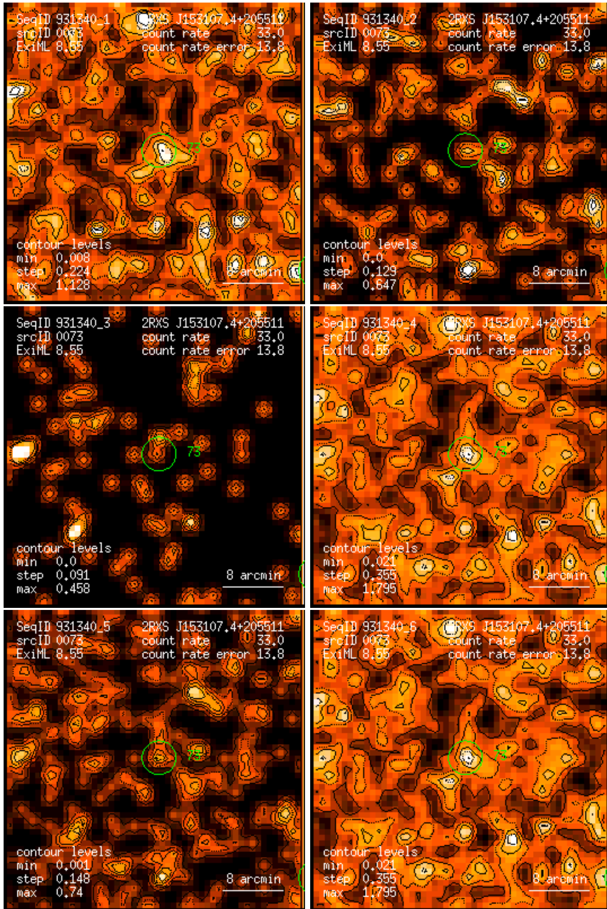
Figure 73: RASS 931340: detection 0073: band rate images, Gaussian filter: (1) PSPC channels 11 – 41, (2) 52 – 90, (3) 91 – 201, (4) 11 – 235, (5) 52 – 201, (6) 11 – 201. Broad band rates in counts/ks. Band rate contour levels in counts/ks/arcmin 2 .
