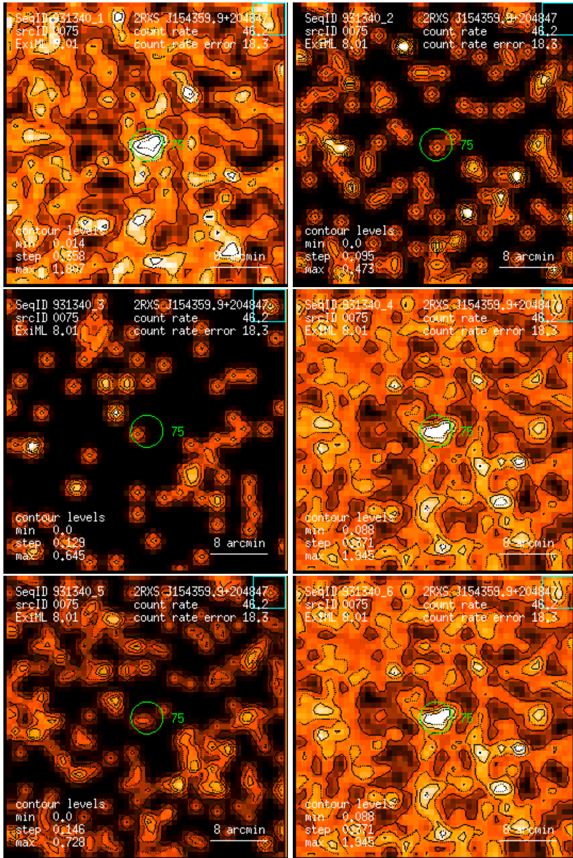
Figure 75: RASS 931340: detection 0075: band rate images, Gaussian filter: (1) PSPC channels 11 – 41, (2) 52 – 90, (3) 91 – 201, (4) 11 – 235, (5) 52 – 201, (6) 11 – 201. Broad band rates in counts/ks. Band rate contour levels in counts/ks/arcmin 2 .
