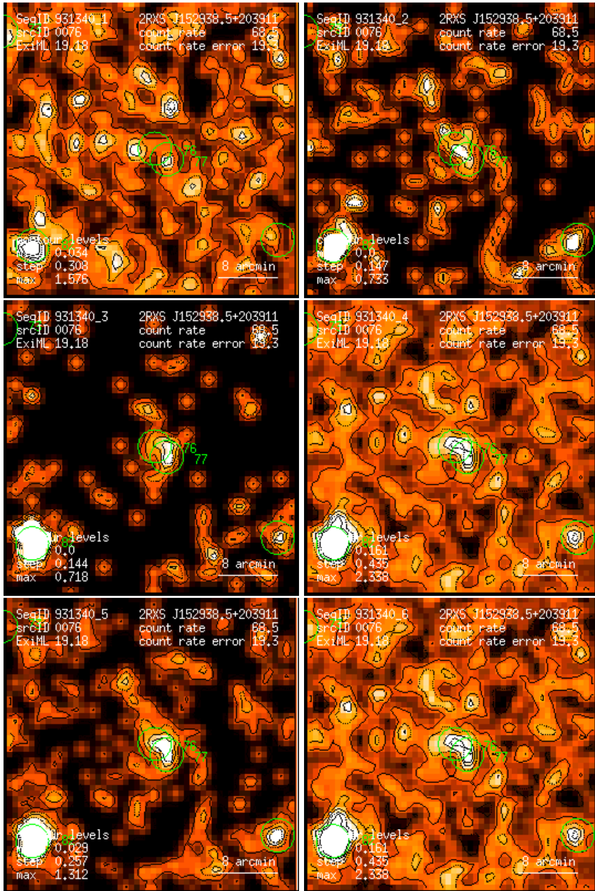
Figure 76: RASS 931340: detection 0076: band rate images, Gaussian filter: (1) PSPC channels 11 – 41, (2) 52 – 90, (3) 91 – 201, (4) 11 – 235, (5) 52 – 201, (6) 11 – 201. Broad band rates in counts/ks. Band rate contour levels in counts/ks/arcmin 2 .
