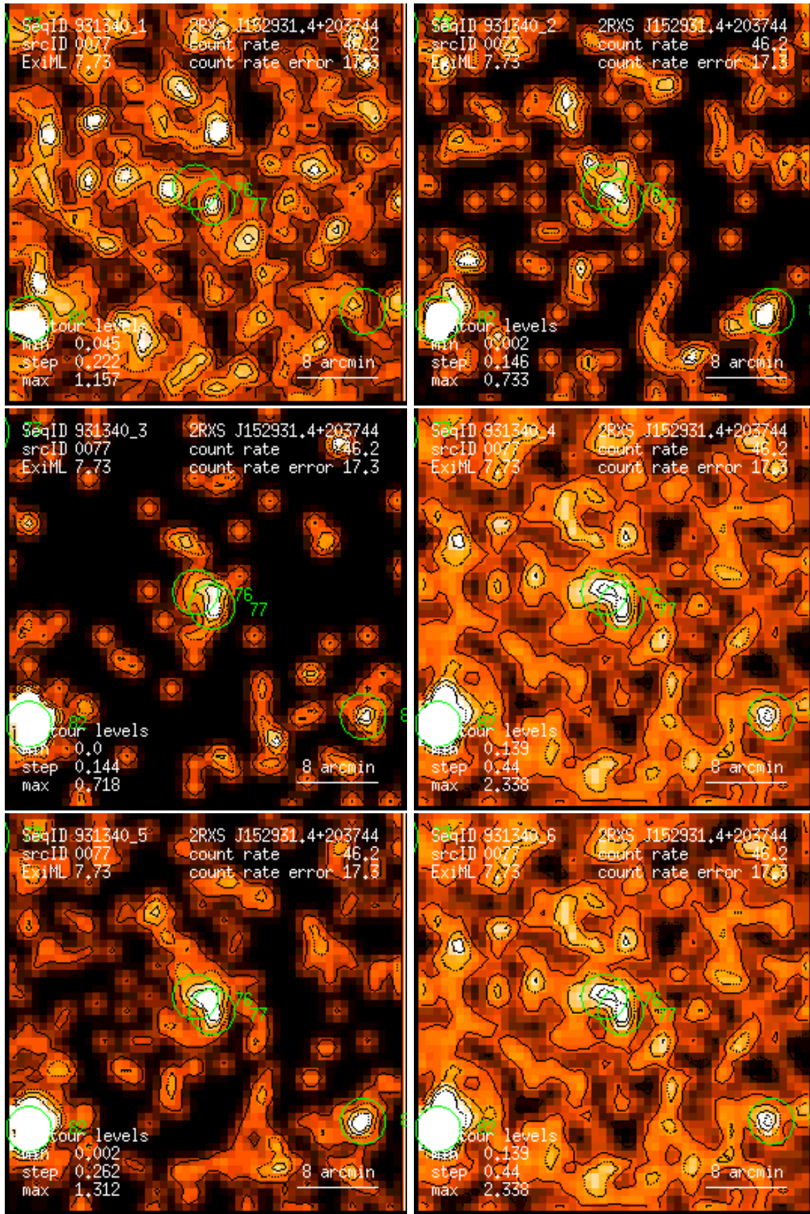
Figure 77: RASS 931340: detection 0077: band rate images, Gaussian filter: (1) PSPC channels 11 – 41, (2) 52 – 90, (3) 91 – 201, (4) 11 – 235, (5) 52 – 201, (6) 11 – 201. Broad band rates in counts/ks. Band rate contour levels in counts/ks/arcmin 2 .
