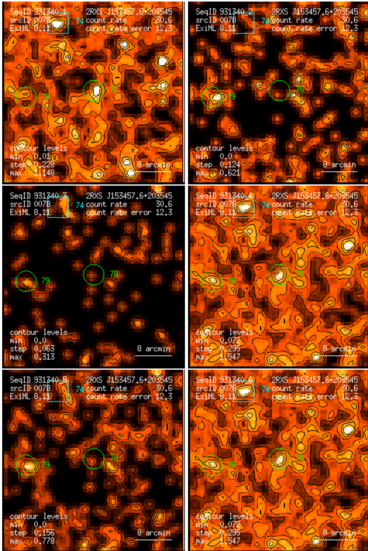
Figure 78: RASS 931340: detection 0078: band rate images, Gaussian filter: (1) PSPC channels 11 – 41, (2) 52 – 90, (3) 91 – 201, (4) 11 – 235, (5) 52 – 201, (6) 11 – 201. Broad band rates in counts/ks. Band rate contour levels in counts/ks/arcmin 2 .
