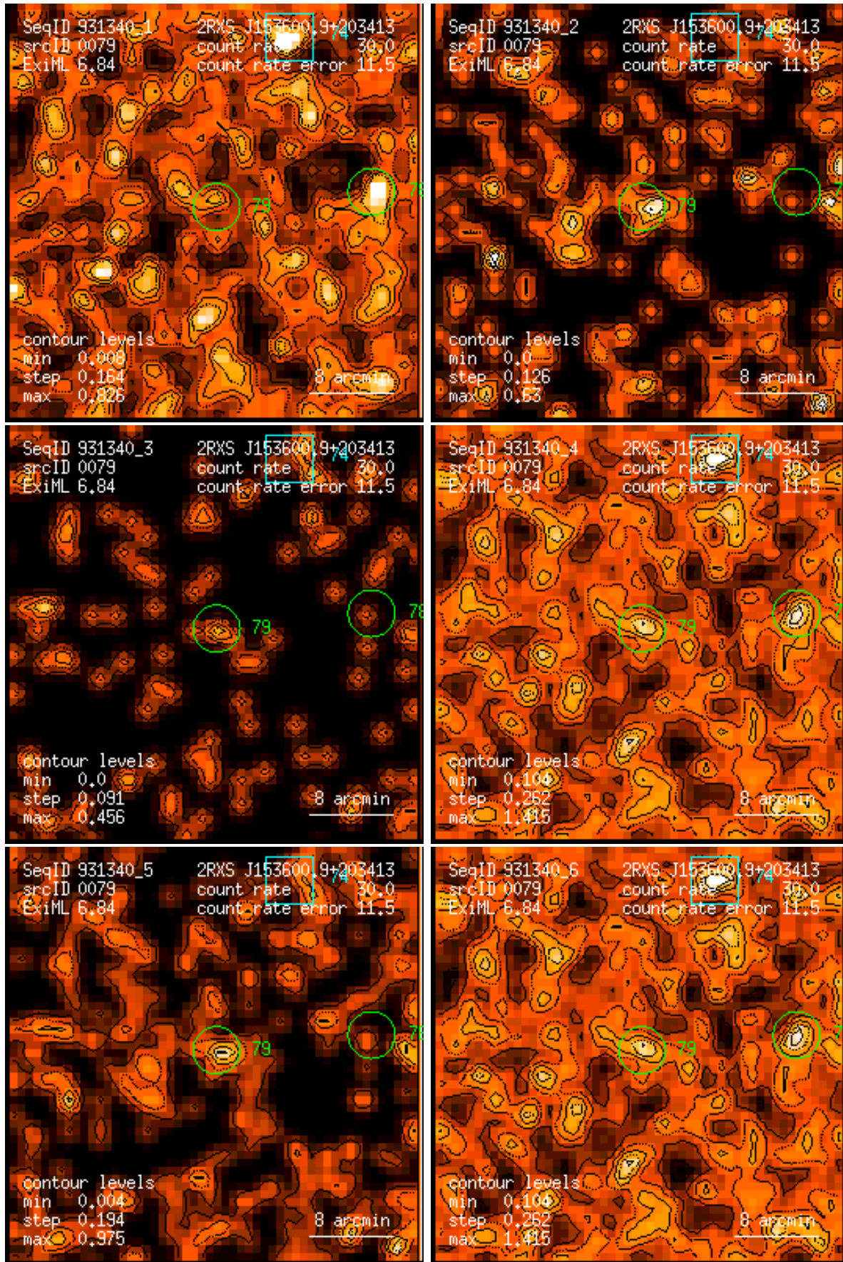
Figure 79: RASS 931340: detection 0079: band rate images, Gaussian filter: (1) PSPC channels 11 – 41, (2) 52 – 90, (3) 91 – 201, (4) 11 – 235, (5) 52 – 201, (6) 11 – 201. Broad band rates in counts/ks. Band rate contour levels in counts/ks/arcmin 2 .
