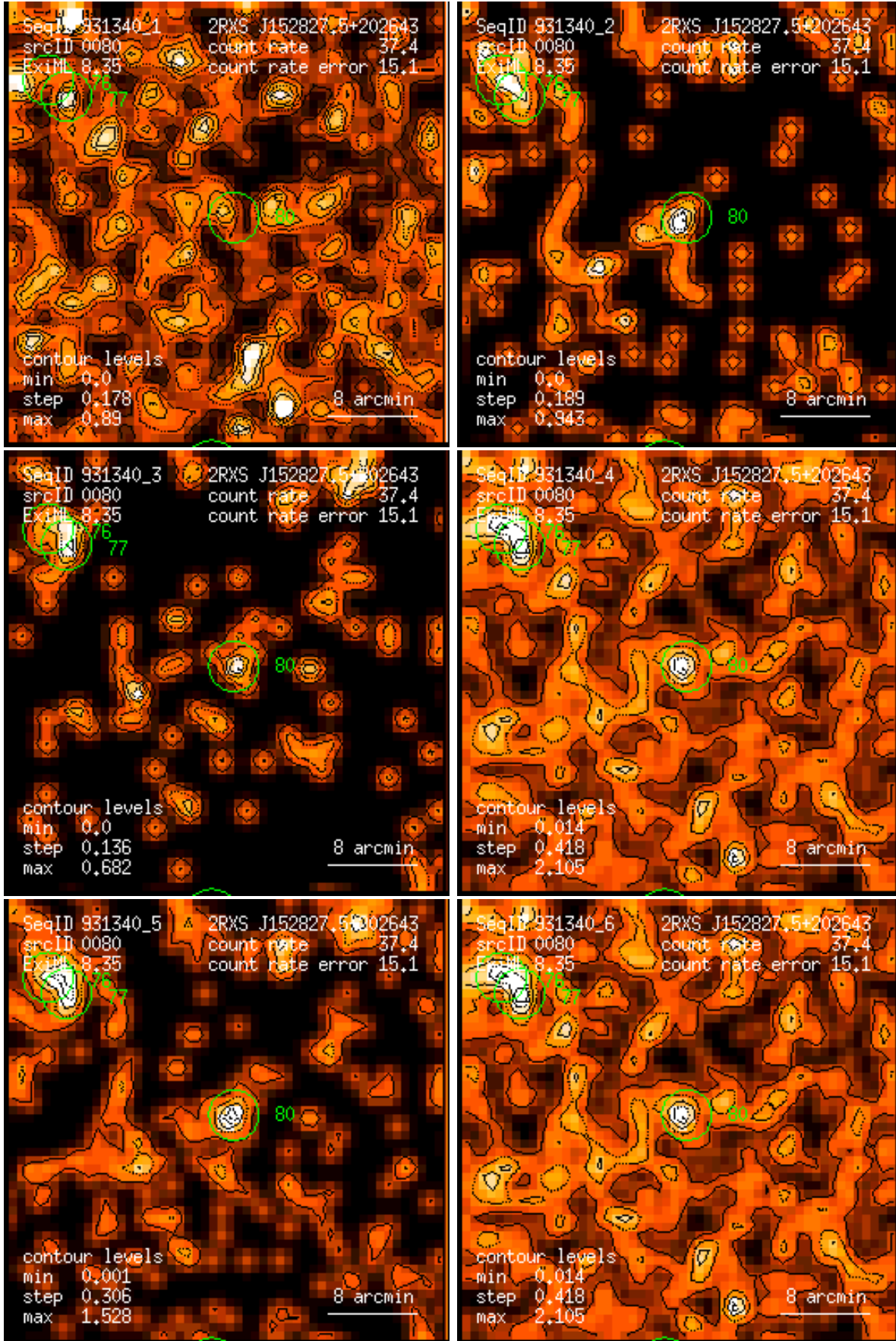
Figure 80: RASS 931340: detection 0080: band rate images, Gaussian filter: (1) PSPC channels 11 – 41, (2) 52 – 90, (3) 91 – 201, (4) 11 – 235, (5) 52 – 201, (6) 11 – 201. Broad band rates in counts/ks. Band rate contour levels in counts/ks/arcmin 2 .
