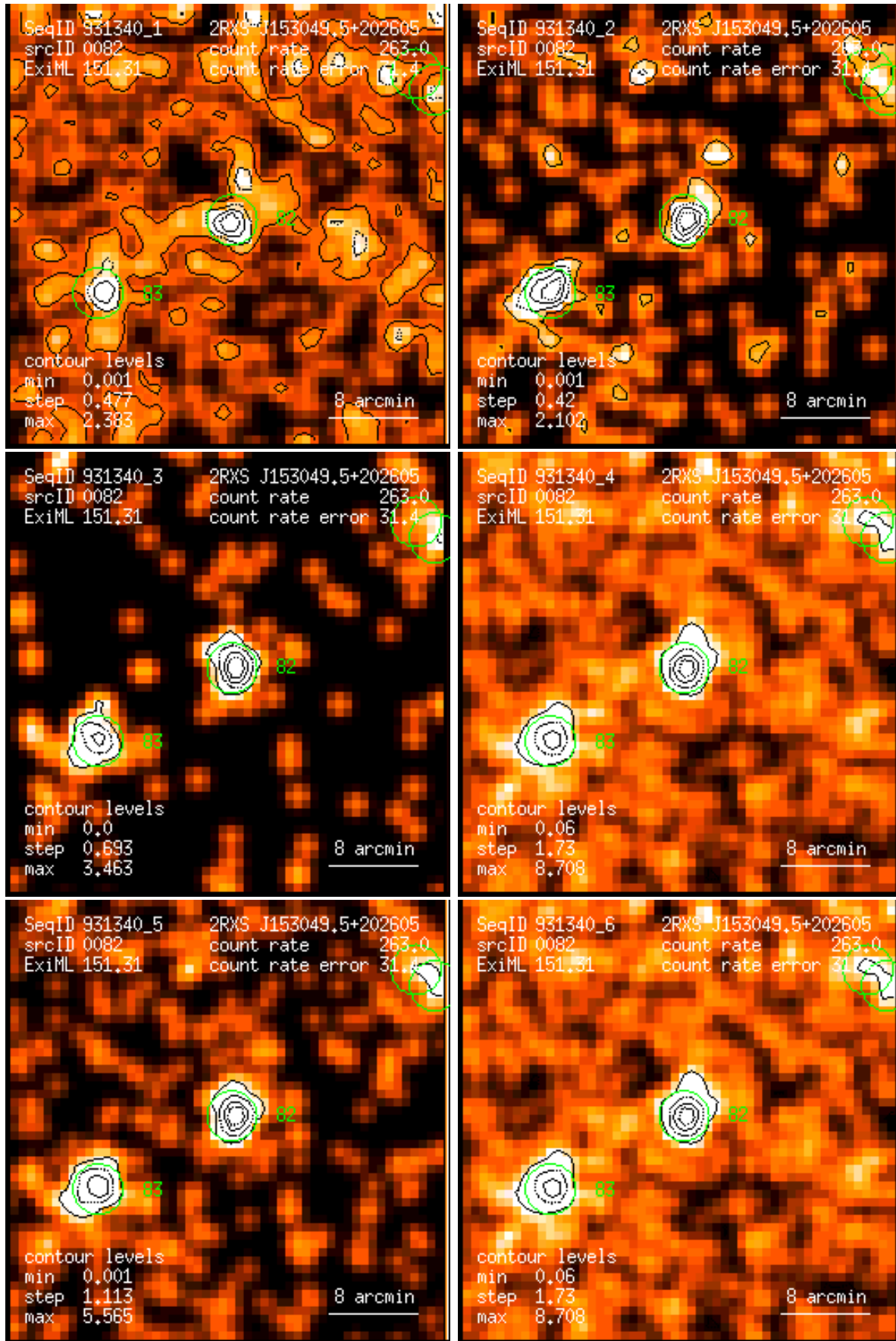
Figure 82: RASS 931340: detection 0082: band rate images, Gaussian filter: (1) PSPC channels 11 – 41, (2) 52 – 90, (3) 91 – 201, (4) 11 – 235, (5) 52 – 201, (6) 11 – 201. Broad band rates in counts/ks. Band rate contour levels in counts/ks/arcmin 2 .
