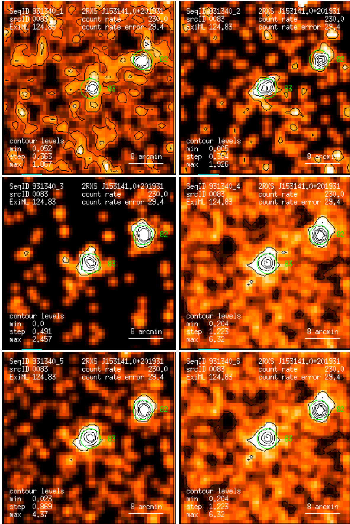
Figure 83: RASS 931340: detection 0083: band rate images, Gaussian filter: (1) PSPC channels 11 – 41, (2) 52 – 90, (3) 91 – 201, (4) 11 – 235, (5) 52 – 201, (6) 11 – 201. Broad band rates in counts/ks. Band rate contour levels in counts/ks/arcmin 2 .
