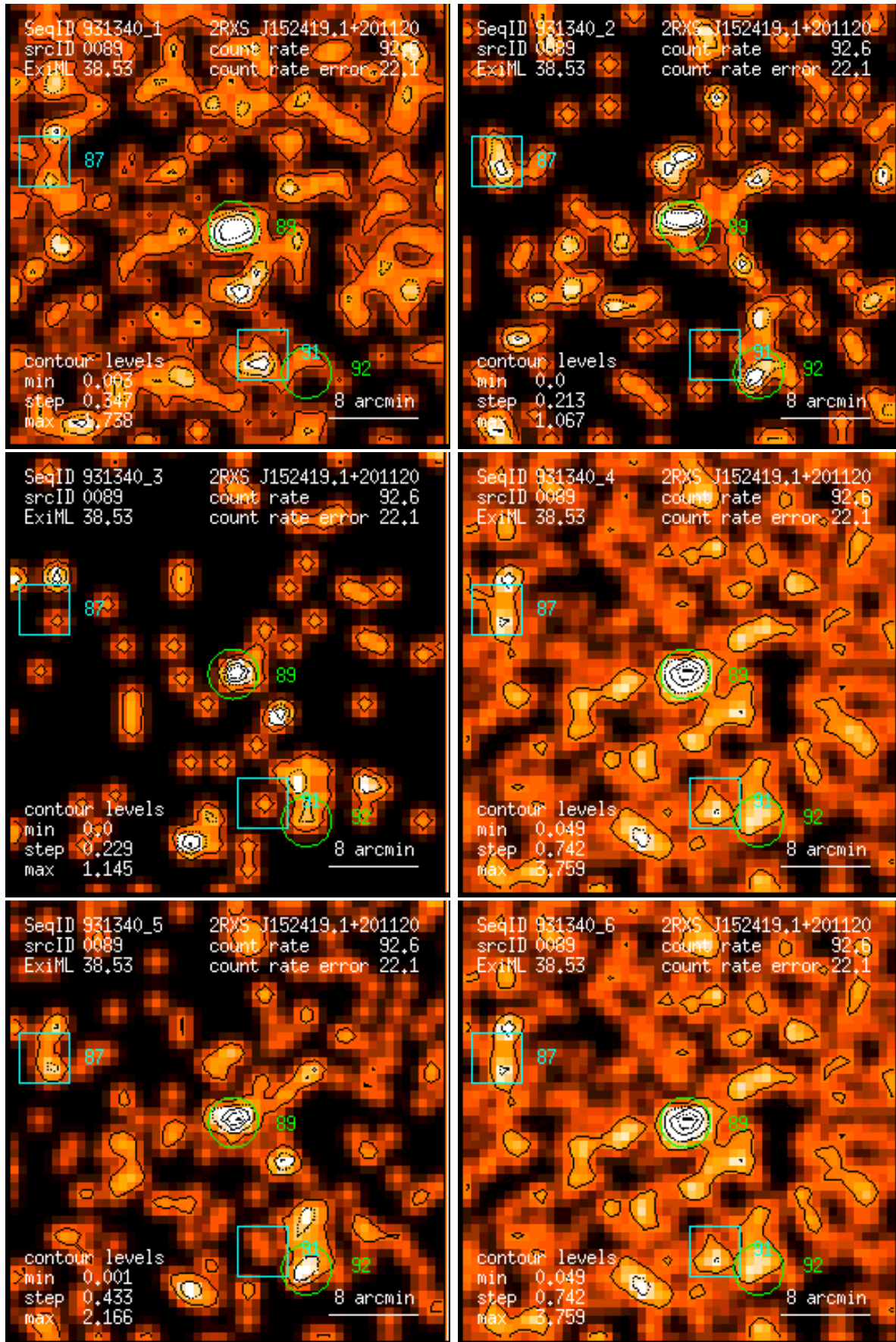
Figure 89: RASS 931340: detection 0089: band rate images, Gaussian filter: (1) PSPC channels 11 – 41, (2) 52 – 90, (3) 91 – 201, (4) 11 – 235, (5) 52 – 201, (6) 11 – 201. Broad band rates in counts/ks. Band rate contour levels in counts/ks/arcmin 2 .
