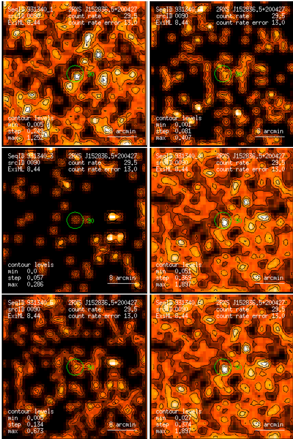
Figure 90: RASS 931340: detection 0090: band rate images, Gaussian filter: (1) PSPC channels 11 – 41, (2) 52 – 90, (3) 91 – 201, (4) 11 – 235, (5) 52 – 201, (6) 11 – 201. Broad band rates in counts/ks. Band rate contour levels in counts/ks/arcmin 2 .
