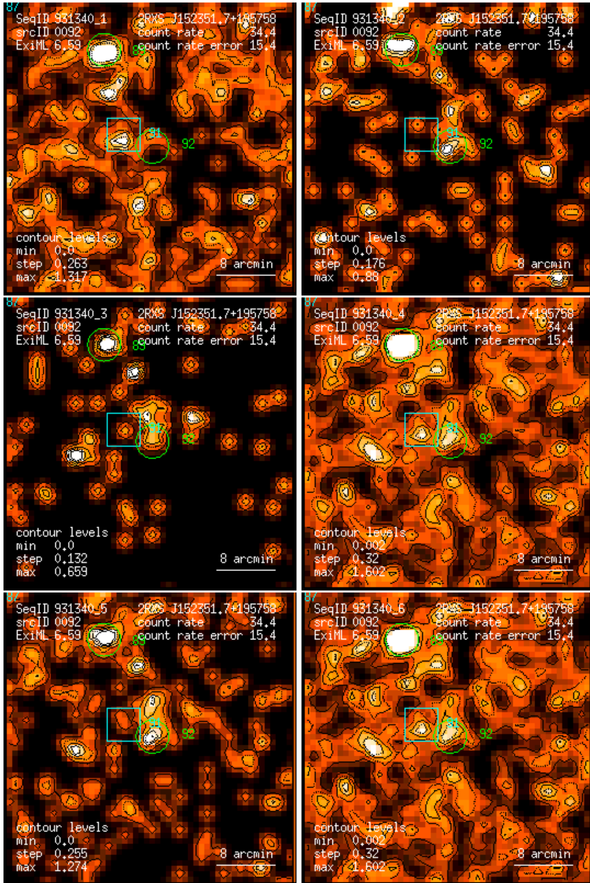
Figure 92: RASS 931340: detection 0092: band rate images, Gaussian filter: (1) PSPC channels 11 – 41, (2) 52 – 90, (3) 91 – 201, (4) 11 – 235, (5) 52 – 201, (6) 11 – 201. Broad band rates in counts/ks. Band rate contour levels in counts/ks/arcmin 2 .
