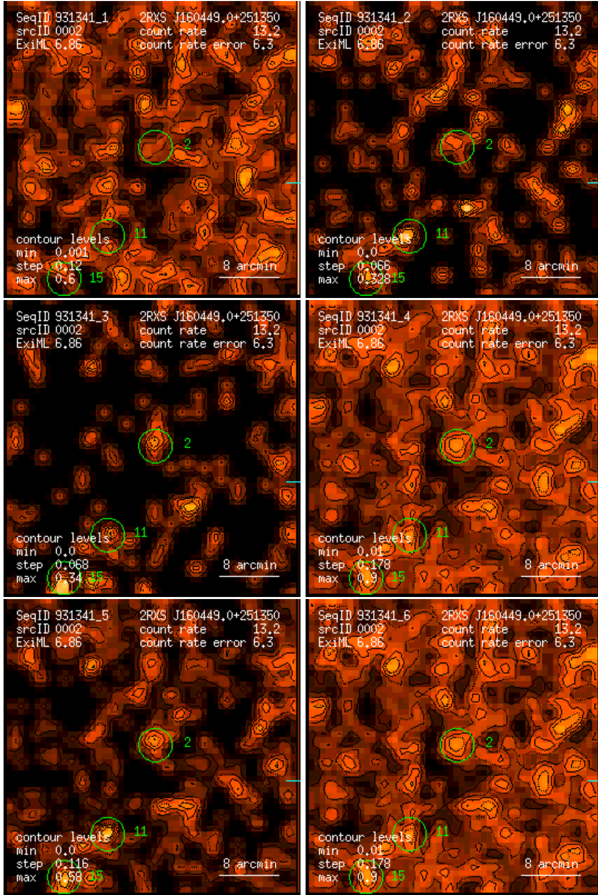
Figure 2: RASS 931341: detection 0002: band rate images, Gaussian filter: (1) PSPC channels 11 – 41, (2) 52 – 90, (3) 91 – 201, (4) 11 – 235, (5) 52 – 201, (6) 11 – 201. Broad band rates in counts/ks. Band rate contour levels in counts/ks/arcmin 2 .
