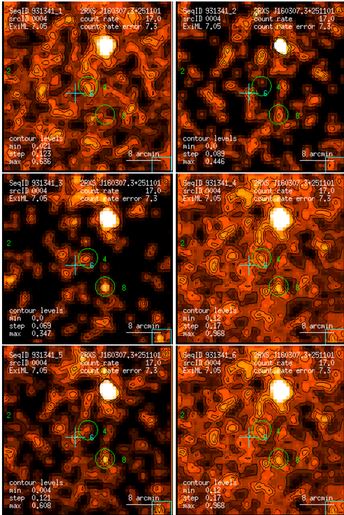
Figure 4: RASS 931341: detection 0004: band rate images, Gaussian filter: (1) PSPC channels 11 – 41, (2) 52 – 90, (3) 91 – 201, (4) 11 – 235, (5) 52 – 201, (6) 11 – 201. Broad band rates in counts/ks. Band rate contour levels in counts/ks/arcmin 2 .
