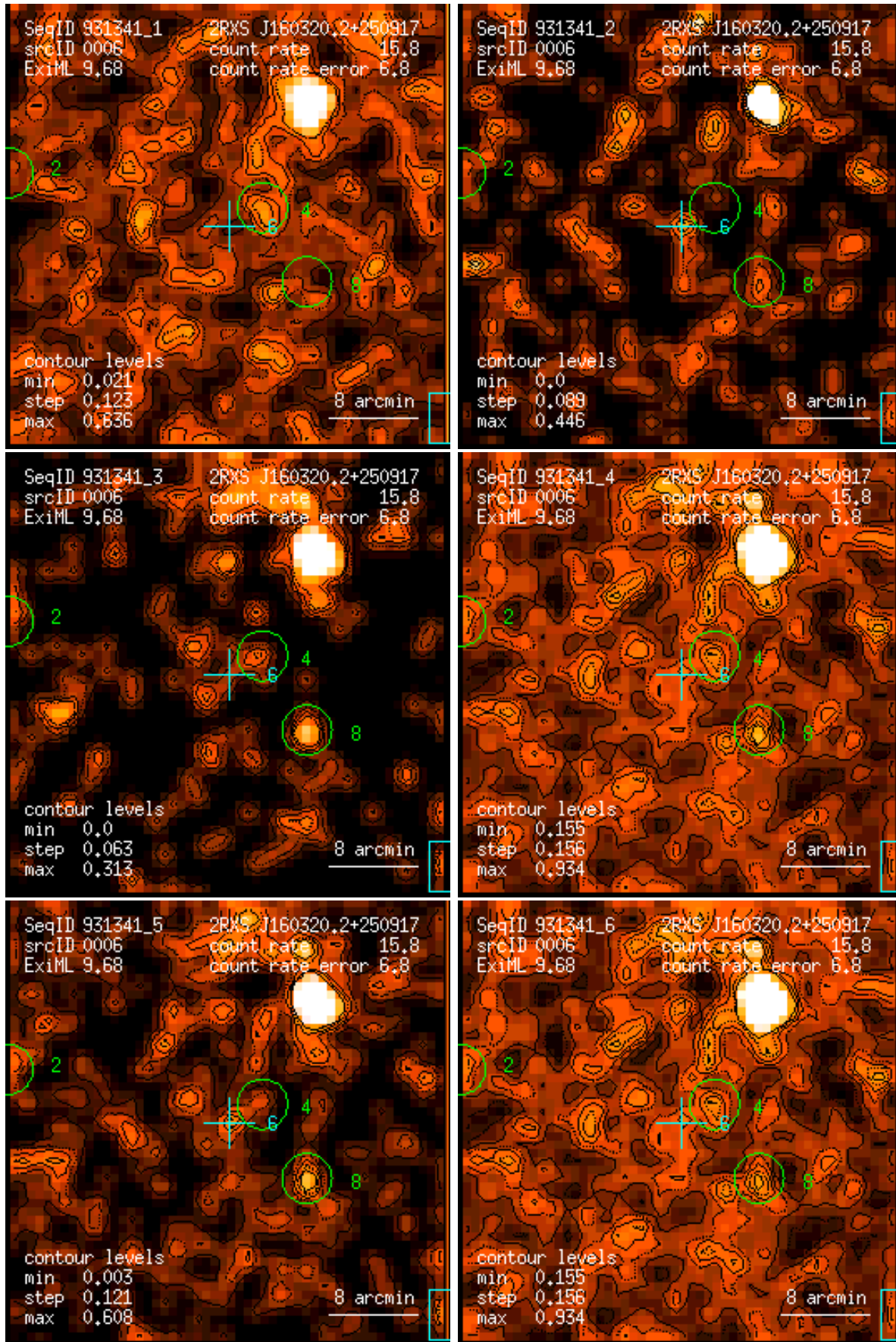
Figure 6: RASS 931341: detection 0006: band rate images, Gaussian filter: (1) PSPC channels 11 – 41, (2) 52 – 90, (3) 91 – 201, (4) 11 – 235, (5) 52 – 201, (6) 11 – 201. Broad band rates in counts/ks. Band rate contour levels in counts/ks/arcmin 2 .
