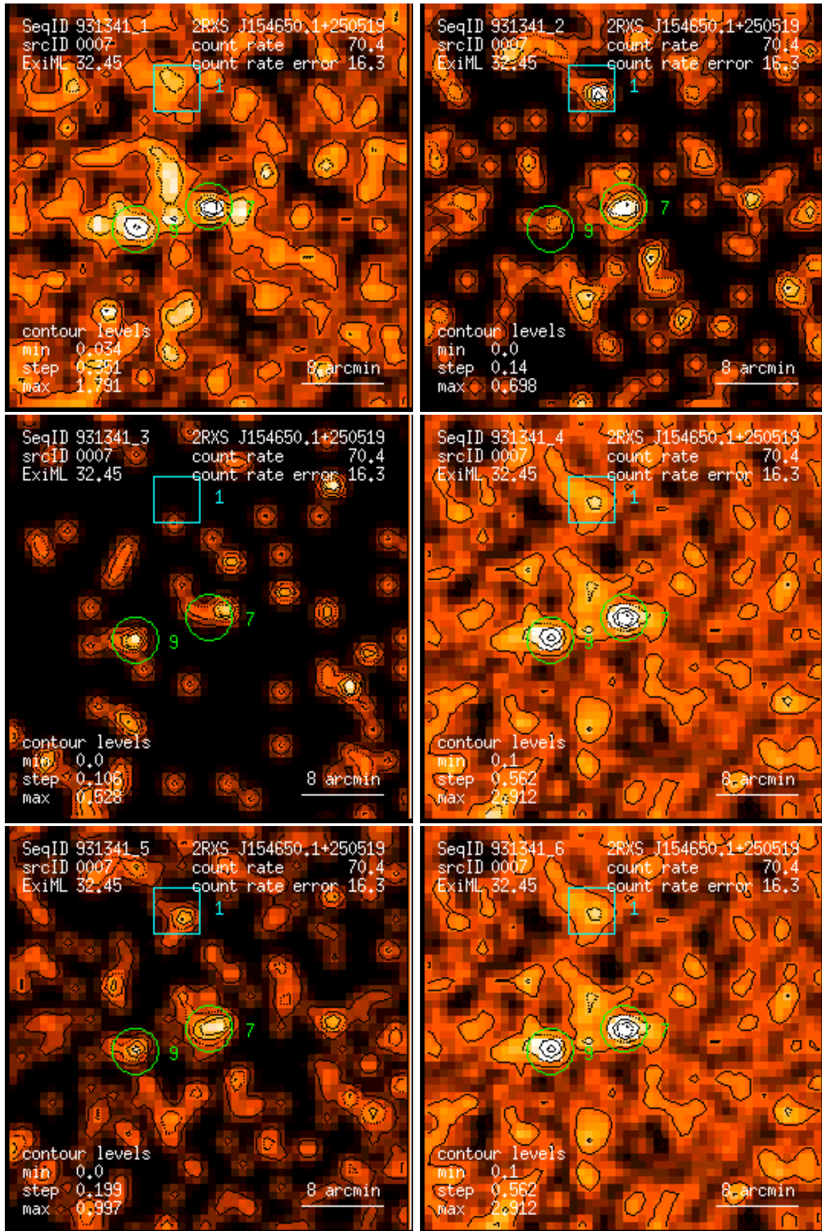
Figure 7: RASS 931341: detection 0007: band rate images, Gaussian filter: (1) PSPC channels 11 – 41, (2) 52 – 90, (3) 91 – 201, (4) 11 – 235, (5) 52 – 201, (6) 11 – 201. Broad band rates in counts/ks. Band rate contour levels in counts/ks/arcmin 2 .
