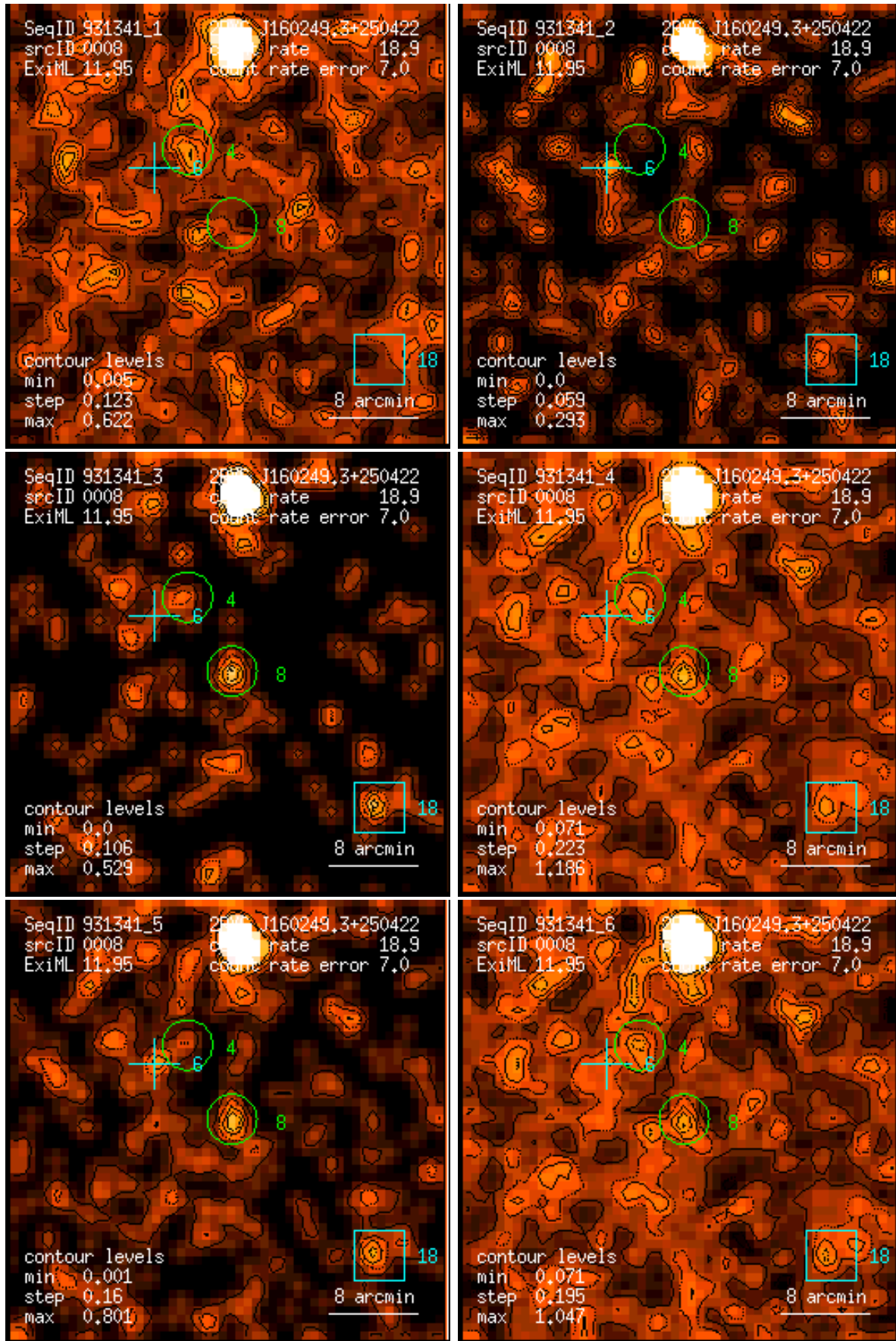
Figure 8: RASS 931341: detection 0008: band rate images, Gaussian filter: (1) PSPC channels 11 – 41, (2) 52 – 90, (3) 91 – 201, (4) 11 – 235, (5) 52 – 201, (6) 11 – 201. Broad band rates in counts/ks. Band rate contour levels in counts/ks/arcmin 2 .
