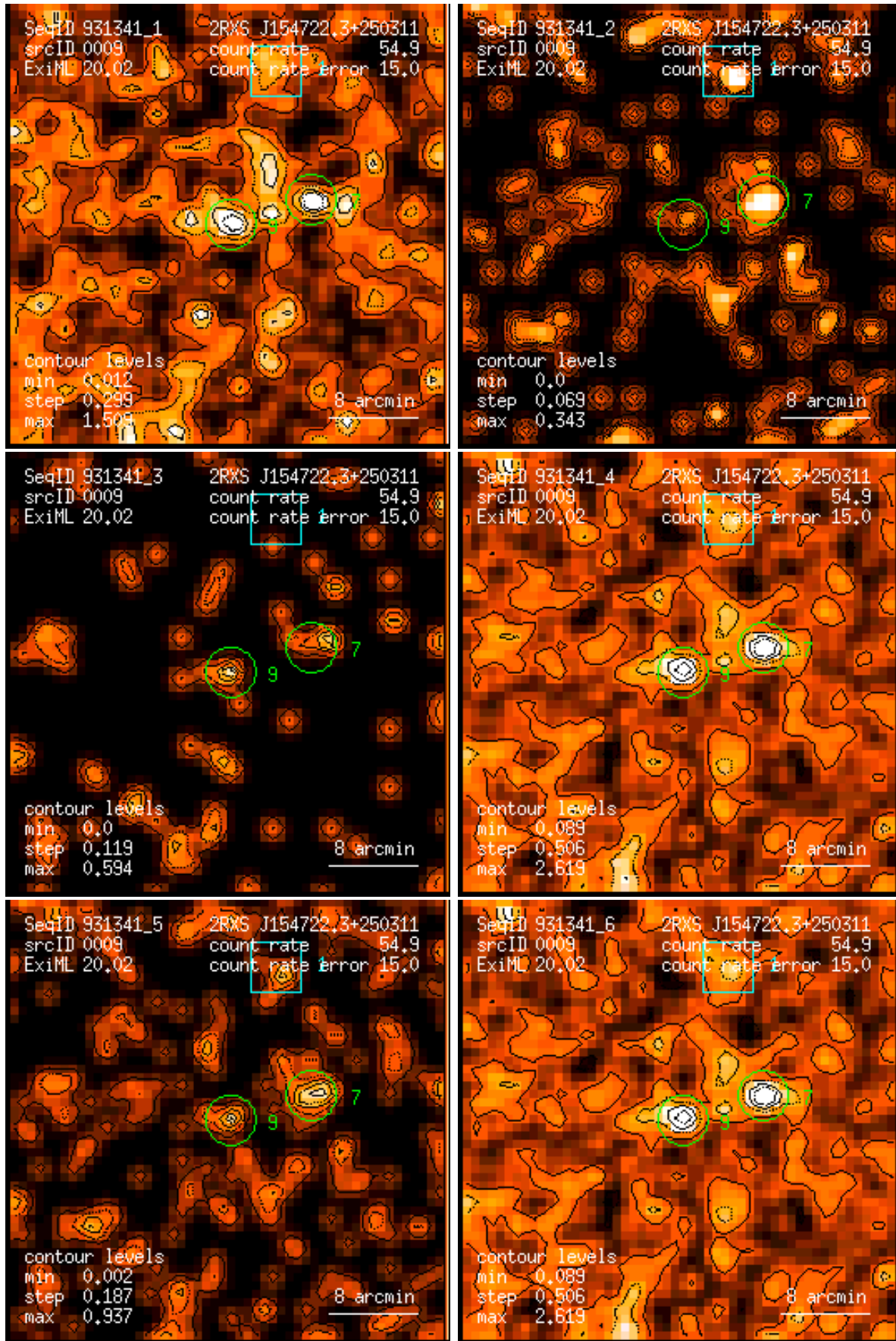
Figure 9: RASS 931341: detection 0009: band rate images, Gaussian filter: (1) PSPC channels 11 – 41, (2) 52 – 90, (3) 91 – 201, (4) 11 – 235, (5) 52 – 201, (6) 11 – 201. Broad band rates in counts/ks. Band rate contour levels in counts/ks/arcmin 2 .
