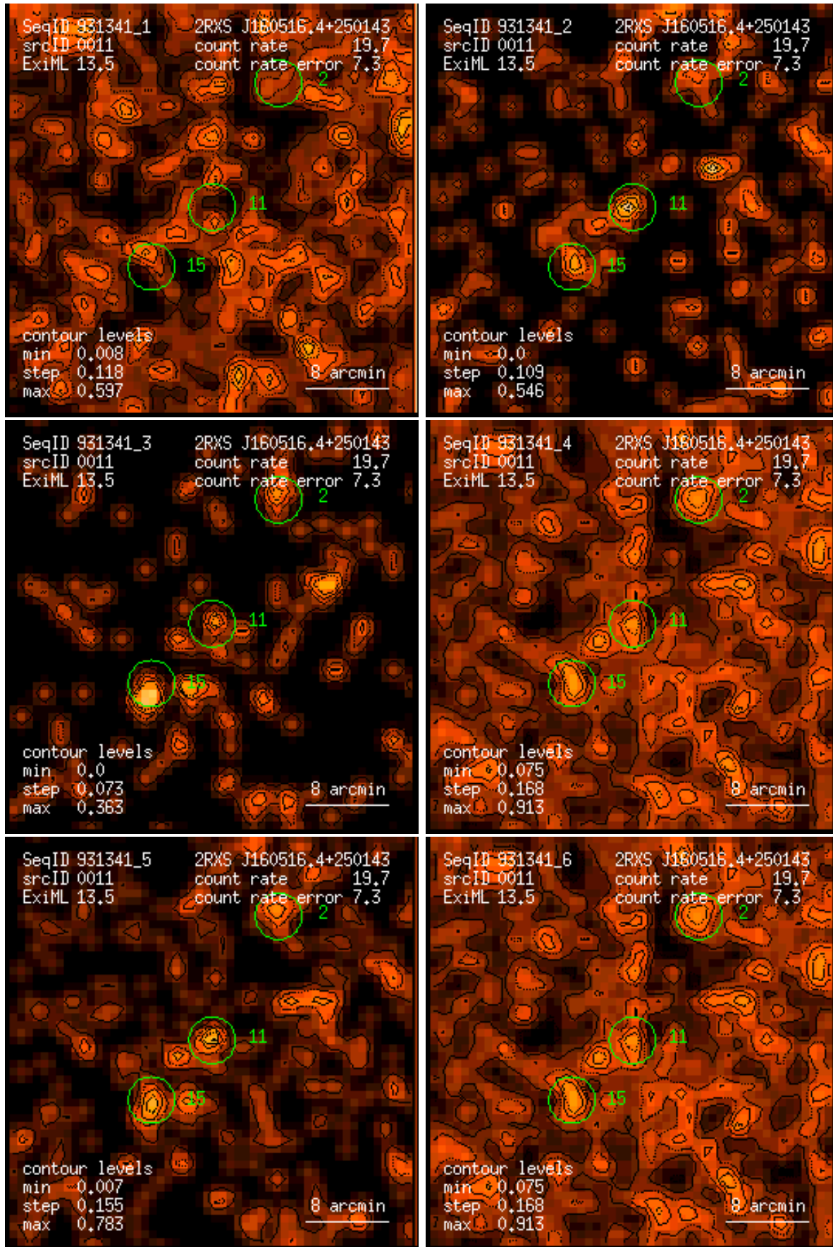
Figure 11: RASS 931341: detection 0011: band rate images, Gaussian filter: (1) PSPC channels 11 – 41, (2) 52 – 90, (3) 91 – 201, (4) 11 – 235, (5) 52 – 201, (6) 11 – 201. Broad band rates in counts/ks. Band rate contour levels in counts/ks/arcmin 2 .
