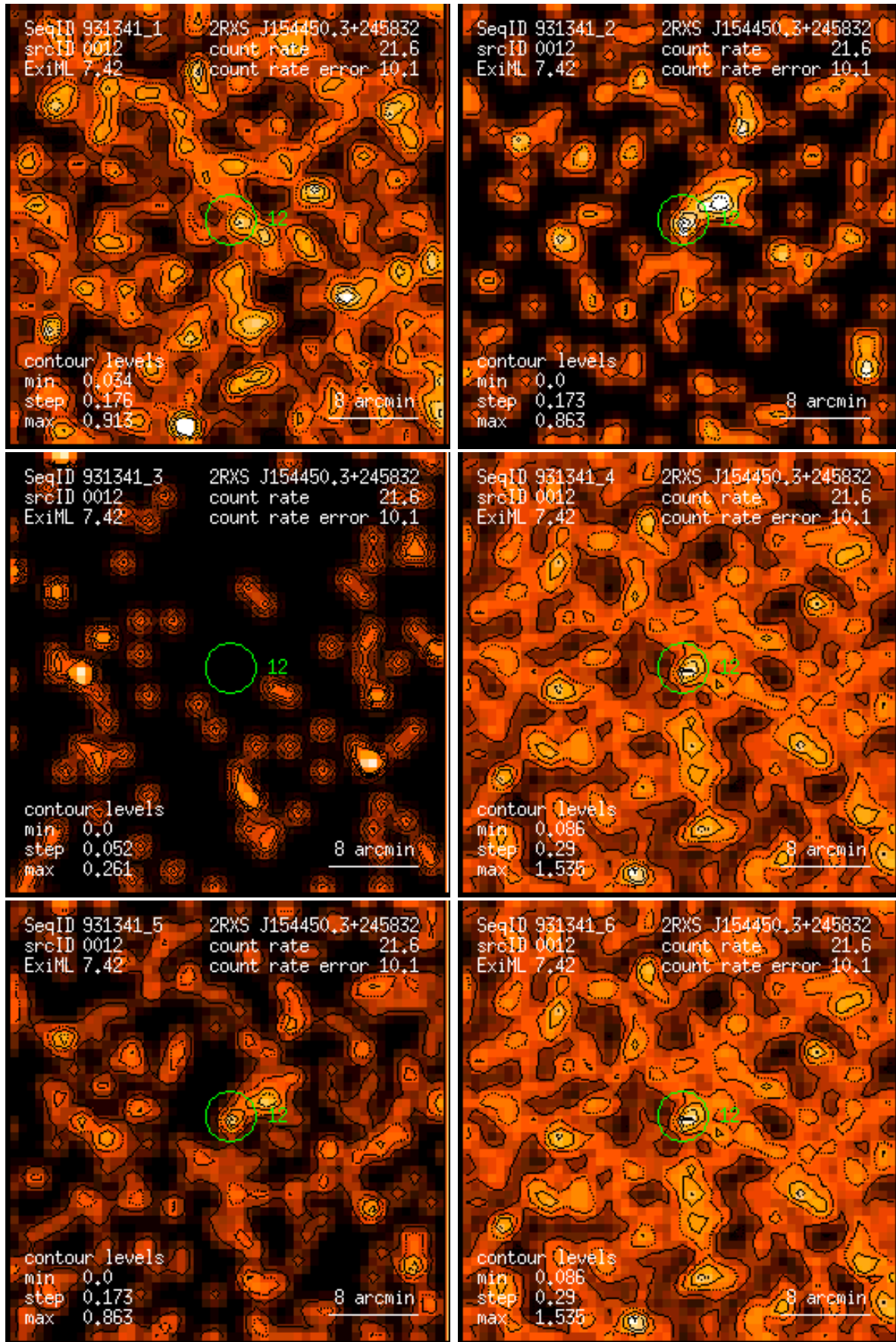
Figure 12: RASS 931341: detection 0012: band rate images, Gaussian filter: (1) PSPC channels 11 – 41, (2) 52 – 90, (3) 91 – 201, (4) 11 – 235, (5) 52 – 201, (6) 11 – 201. Broad band rates in counts/ks. Band rate contour levels in counts/ks/arcmin 2 .
