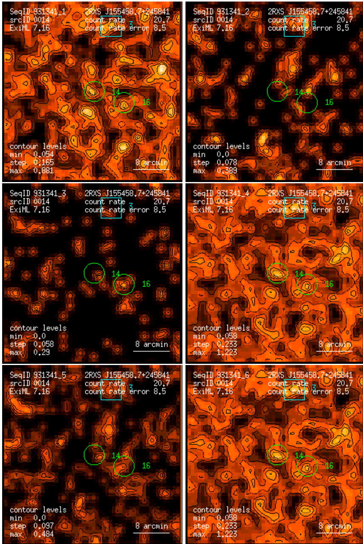
Figure 14: RASS 931341: detection 0014: band rate images, Gaussian filter: (1) PSPC channels 11 – 41, (2) 52 – 90, (3) 91 – 201, (4) 11 – 235, (5) 52 – 201, (6) 11 – 201. Broad band rates in counts/ks. Band rate contour levels in counts/ks/arcmin 2 .
