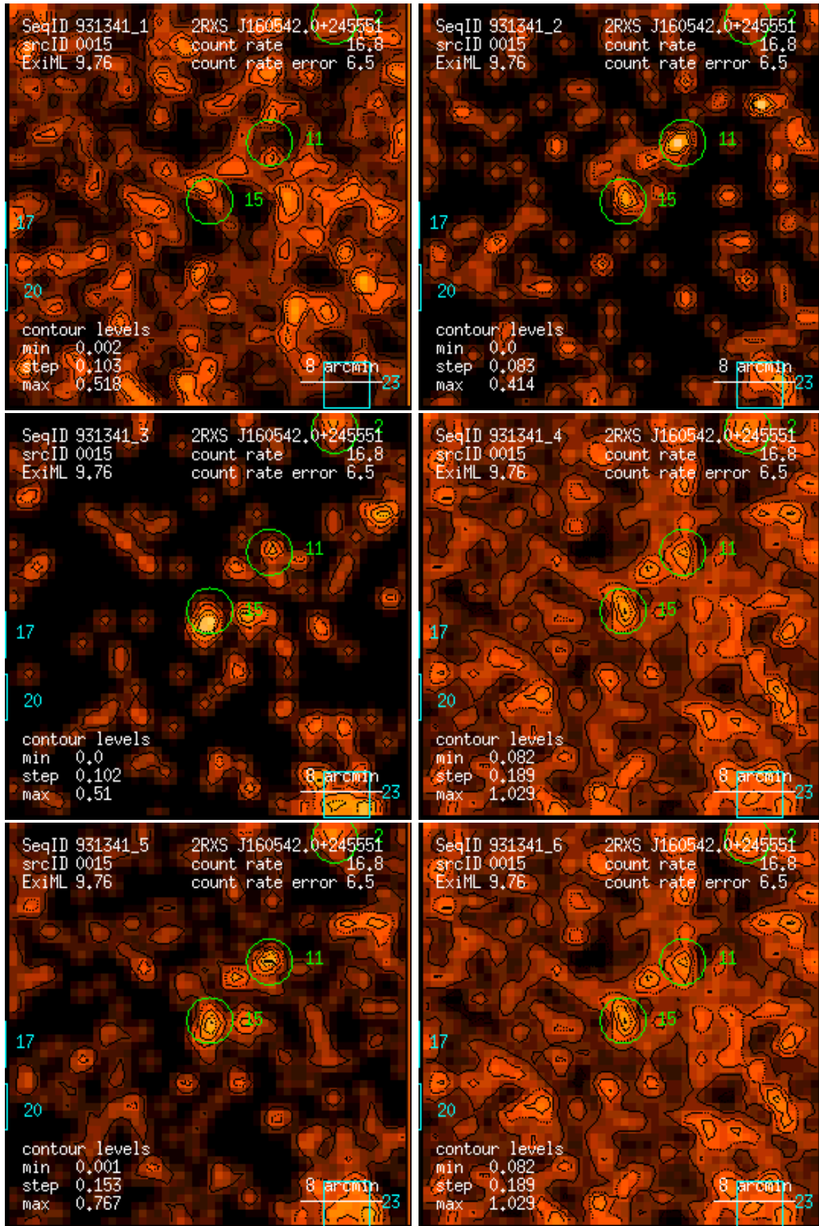
Figure 15: RASS 931341: detection 0015: band rate images, Gaussian filter: (1) PSPC channels 11 – 41, (2) 52 – 90, (3) 91 – 201, (4) 11 – 235, (5) 52 – 201, (6) 11 – 201. Broad band rates in counts/ks. Band rate contour levels in counts/ks/arcmin 2 .
