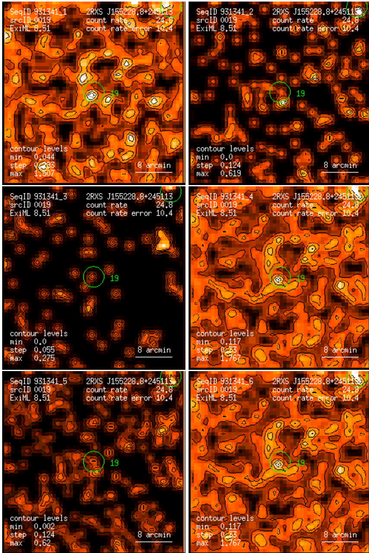
Figure 19: RASS 931341: detection 0019: band rate images, Gaussian filter: (1) PSPC channels 11 – 41, (2) 52 – 90, (3) 91 – 201, (4) 11 – 235, (5) 52 – 201, (6) 11 – 201. Broad band rates in counts/ks. Band rate contour levels in counts/ks/arcmin 2 .
