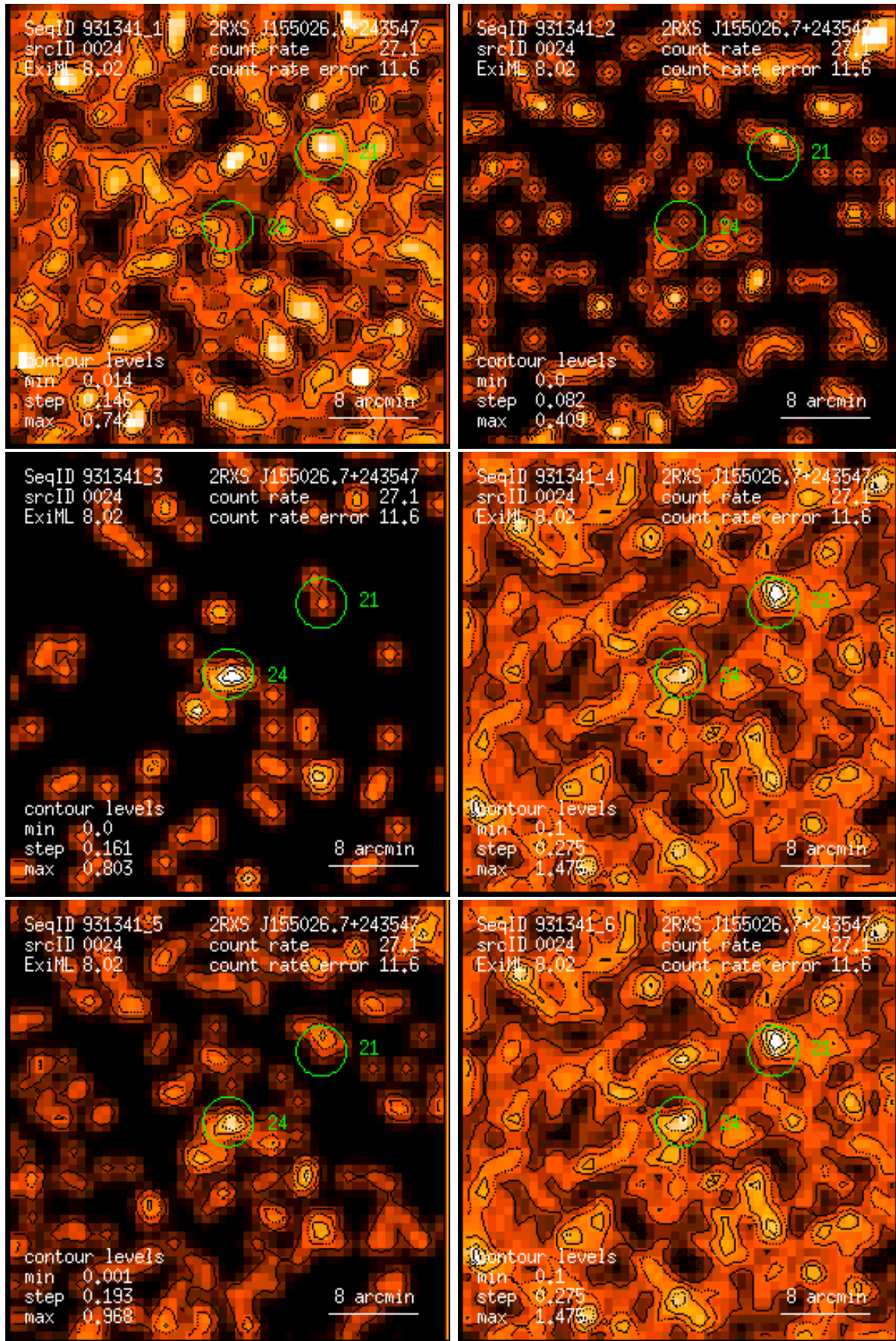
Figure 24: RASS 931341: detection 0024: band rate images, Gaussian filter: (1) PSPC channels 11 – 41, (2) 52 – 90, (3) 91 – 201, (4) 11 – 235, (5) 52 – 201, (6) 11 – 201. Broad band rates in counts/ks. Band rate contour levels in counts/ks/arcmin 2 .
