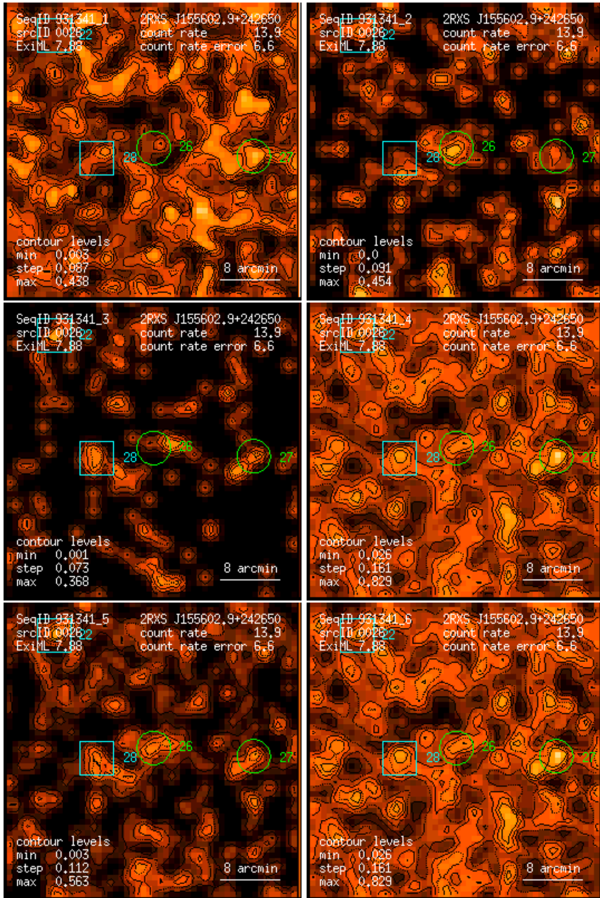
Figure 26: RASS 931341: detection 0026: band rate images, Gaussian filter: (1) PSPC channels 11 – 41, (2) 52 – 90, (3) 91 – 201, (4) 11 – 235, (5) 52 – 201, (6) 11 – 201. Broad band rates in counts/ks. Band rate contour levels in counts/ks/arcmin 2 .
