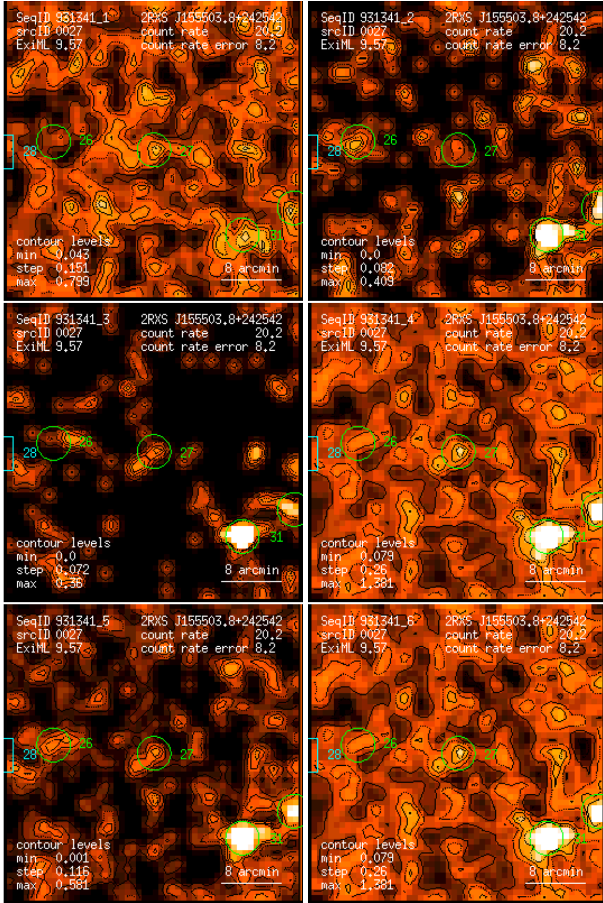
Figure 27: RASS 931341: detection 0027: band rate images, Gaussian filter: (1) PSPC channels 11 – 41, (2) 52 – 90, (3) 91 – 201, (4) 11 – 235, (5) 52 – 201, (6) 11 – 201. Broad band rates in counts/ks. Band rate contour levels in counts/ks/arcmin 2 .
