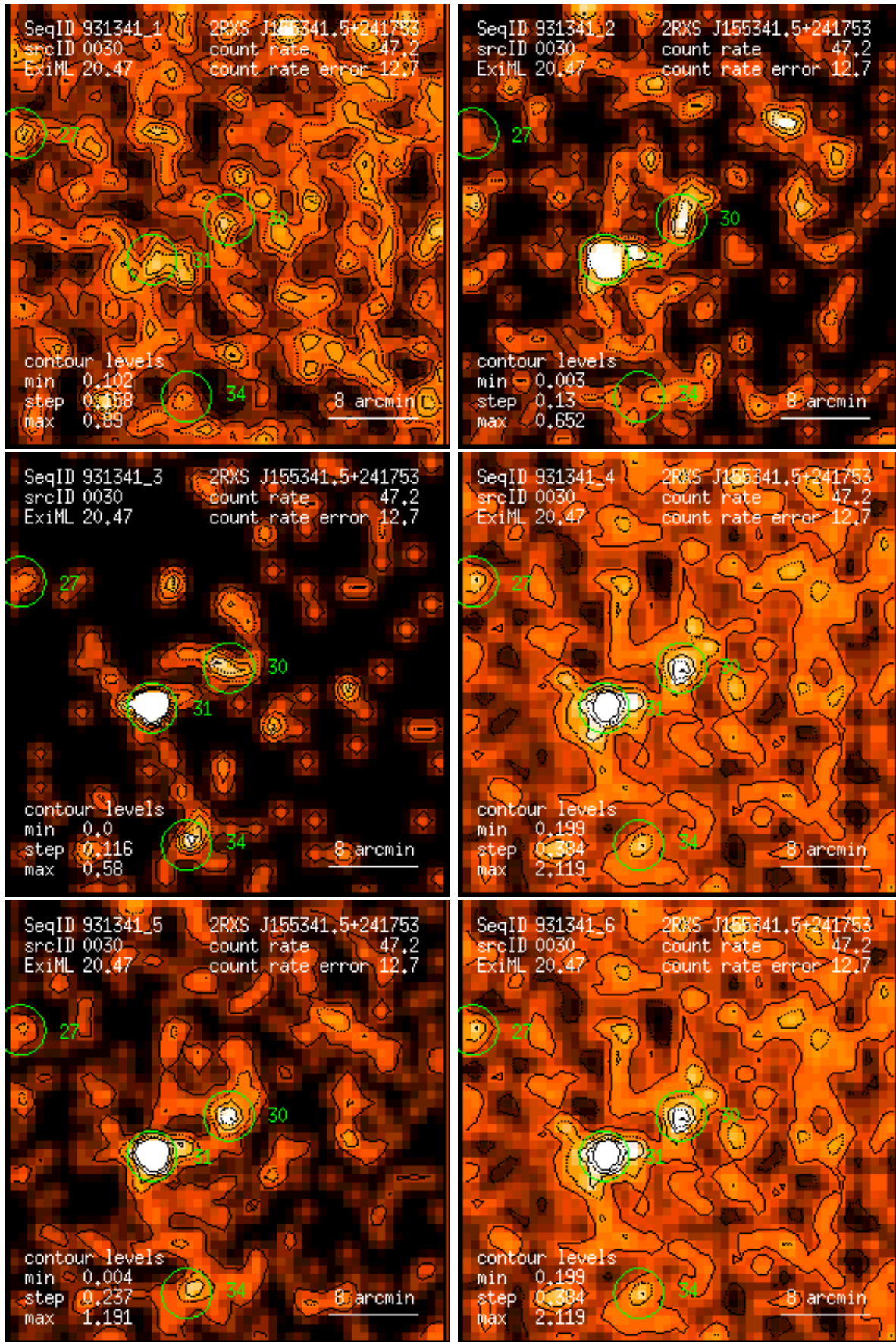
Figure 30: RASS 931341: detection 0030: band rate images, Gaussian filter: (1) PSPC channels 11 – 41, (2) 52 – 90, (3) 91 – 201, (4) 11 – 235, (5) 52 – 201, (6) 11 – 201. Broad band rates in counts/ks. Band rate contour levels in counts/ks/arcmin 2 .
