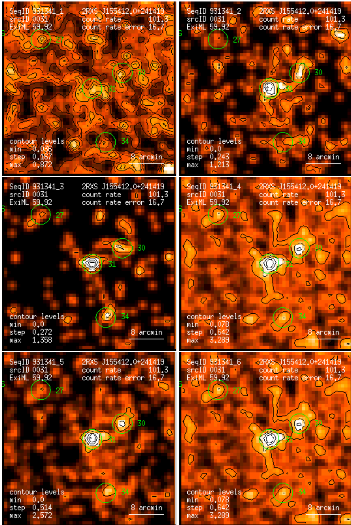
Figure 31: RASS 931341: detection 0031: band rate images, Gaussian filter: (1) PSPC channels 11 – 41, (2) 52 – 90, (3) 91 – 201, (4) 11 – 235, (5) 52 – 201, (6) 11 – 201. Broad band rates in counts/ks. Band rate contour levels in counts/ks/arcmin 2 .
