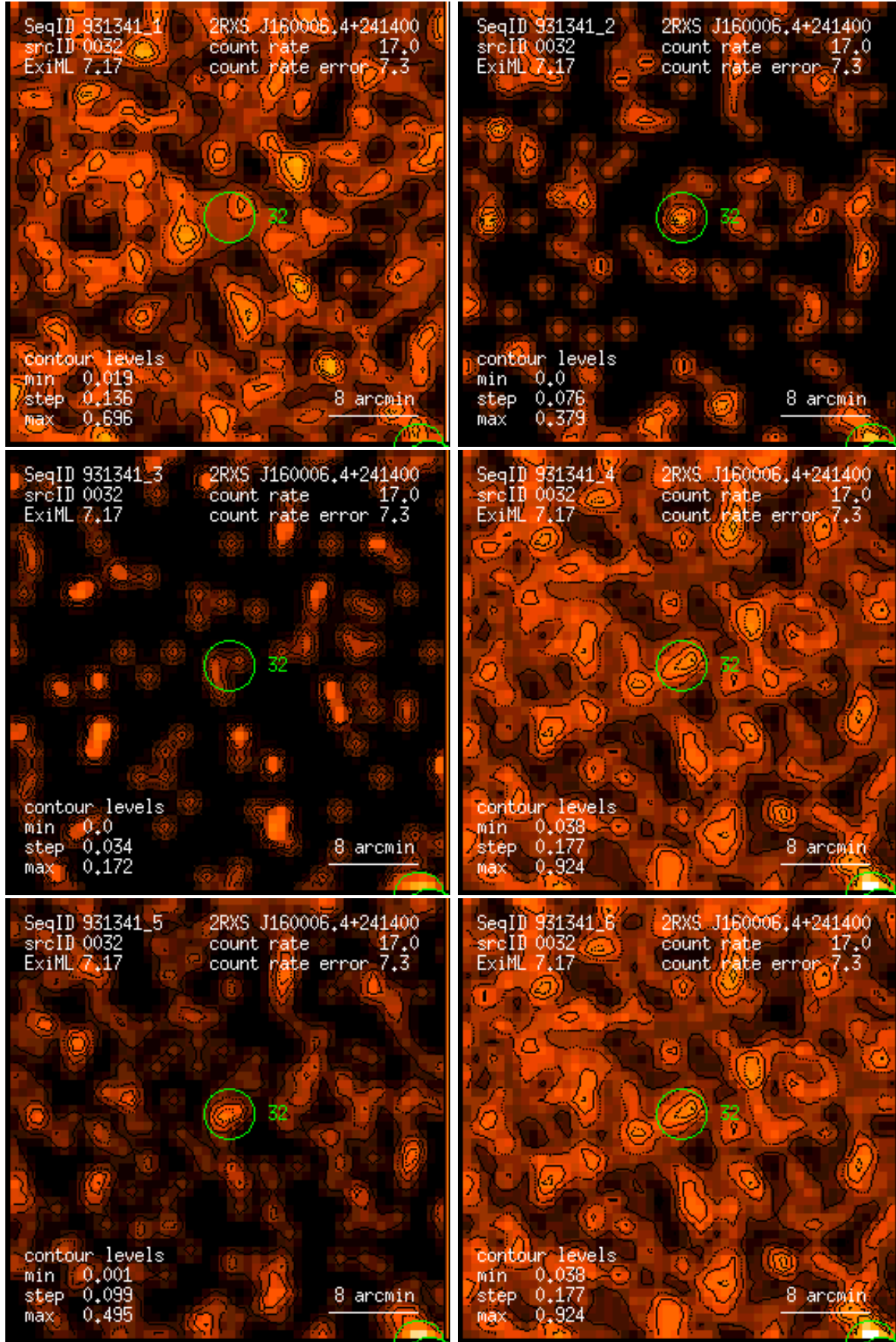
Figure 32: RASS 931341: detection 0032: band rate images, Gaussian filter: (1) PSPC channels 11 – 41, (2) 52 – 90, (3) 91 – 201, (4) 11 – 235, (5) 52 – 201, (6) 11 – 201. Broad band rates in counts/ks. Band rate contour levels in counts/ks/arcmin 2 .
